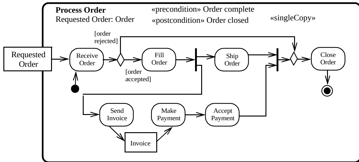
Figure 203 - Example of an activity with input parameter
