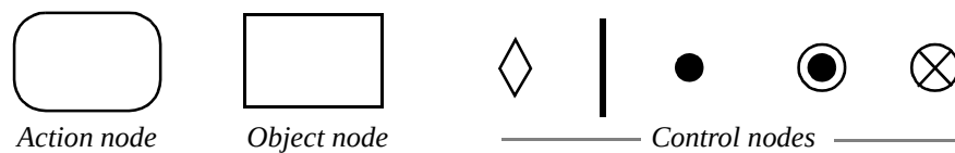
Figure 218 - Activity node notation
