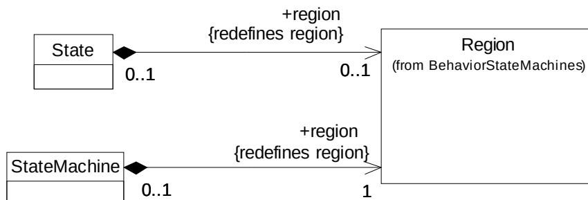
Figure 358 - StatesMachines and States with maximum one region
