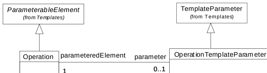
Figure 441 - Operation template parameters
