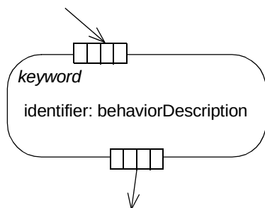
Figure 243 - Shorthand notation for expansion region containing single node
