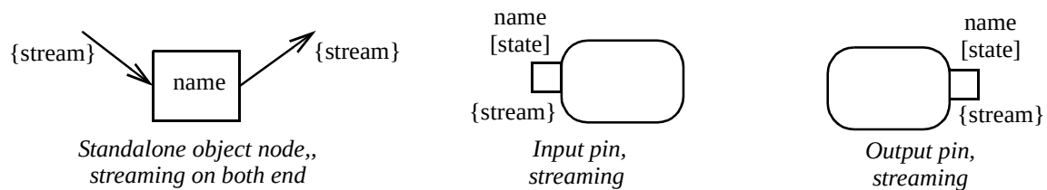
Figure 282 - Stream pin notations
