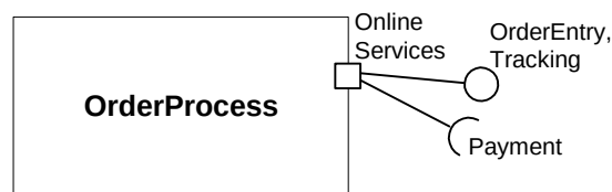
Figure 112 - Port notation showing multiple provided interfaces
