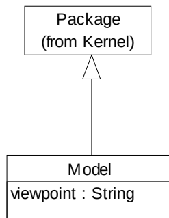
Figure 419 - The contents of the Models package
