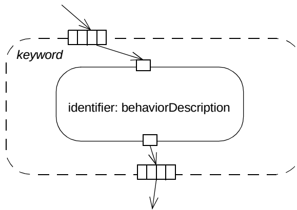
Figure 244 - Full form of previous shorthand notation
