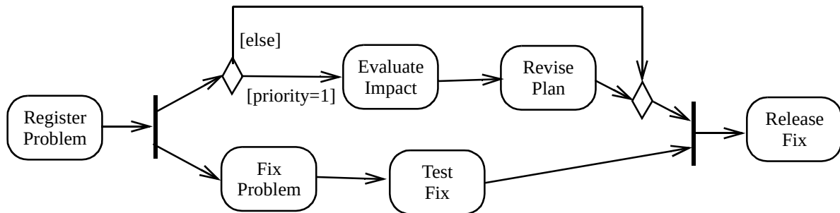
Figure 212 - Equivalent model to Figure 211
