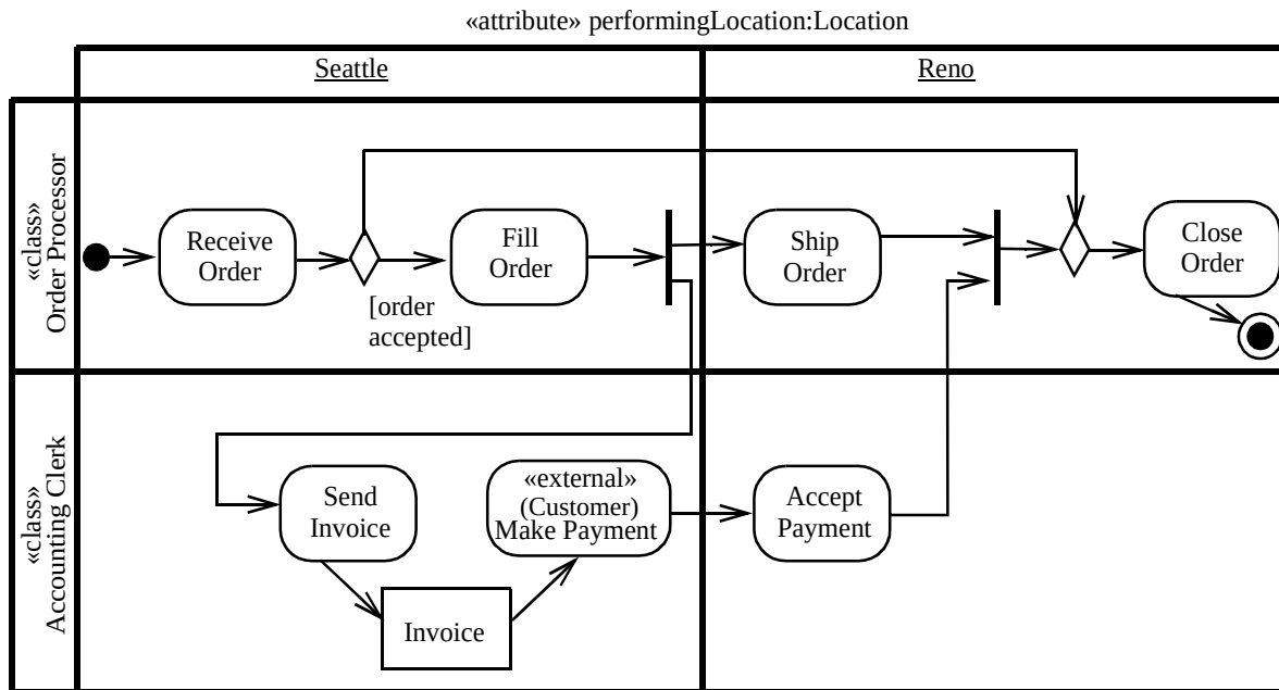
Figure 228 - Activity partition using multidimensional swimlane example
