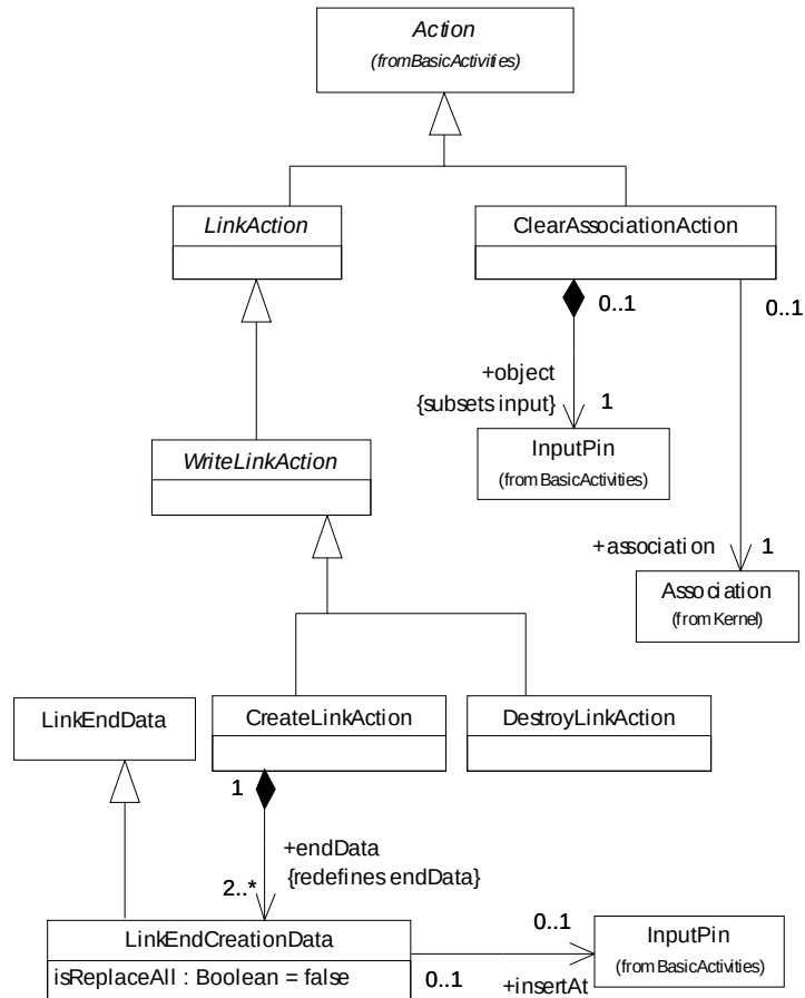
Figure 148 - Write link actions
