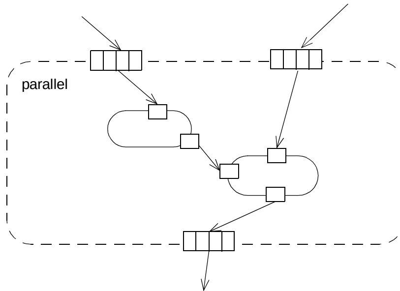
Figure 246 - Expansion region with 2 inputs and 1 output
