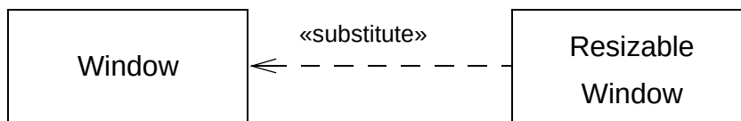
Figure 56 - An example of a substitute dependency
