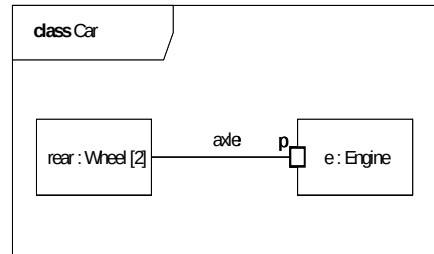
ii) Composite structure diagram for the same class Car
