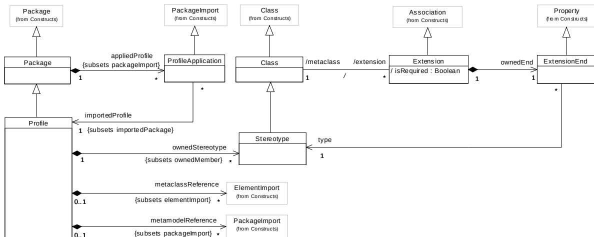
Figure 446 - The elements defined in the Profiles package
