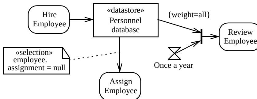
Figure 236 - Data store node example
