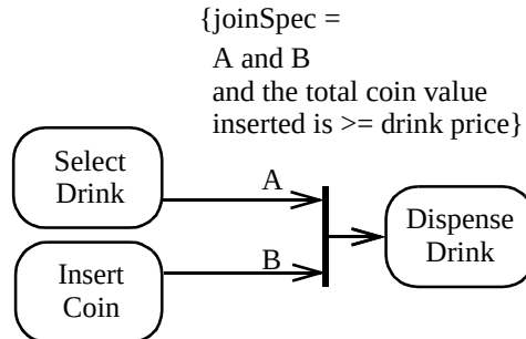
Figure 264 - Join node example
