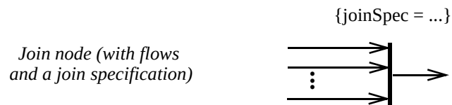
Figure 262 - Join node notations
