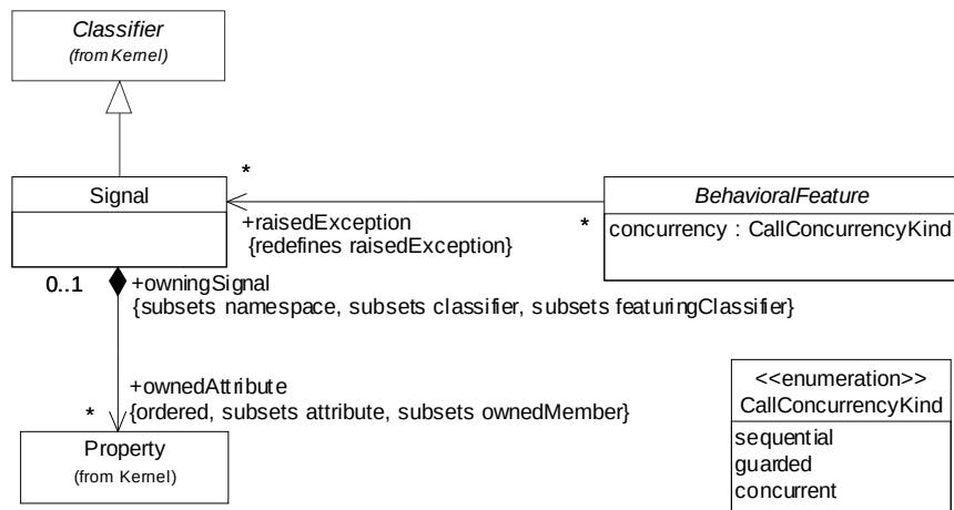
Figure 316 - Extensions to behavioral features and signal
