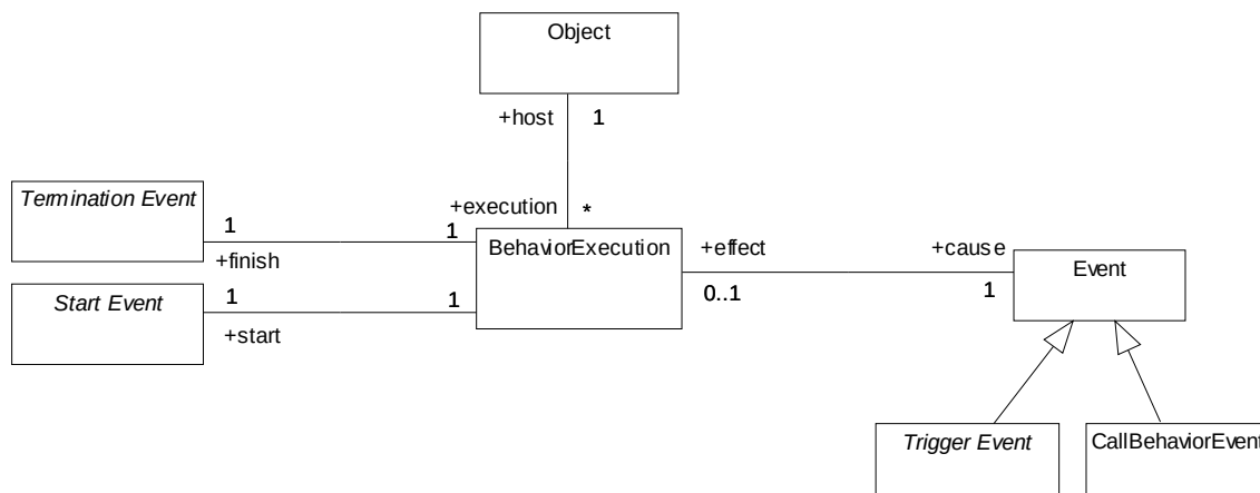
Figure 307 - Invocation Domain Model
