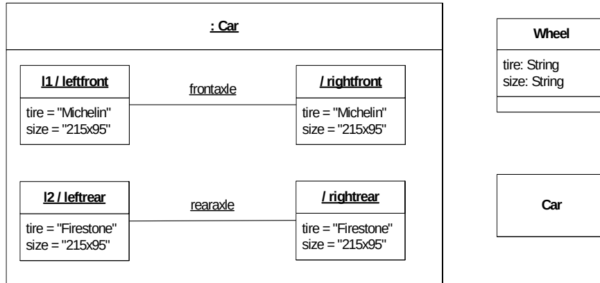
Figure 120 - A instance of the Car class
