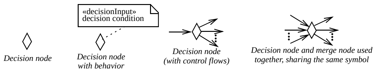
Figure 237 - Decision node notation
