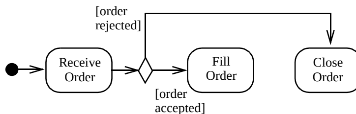
Figure 238 - Decision node example.
