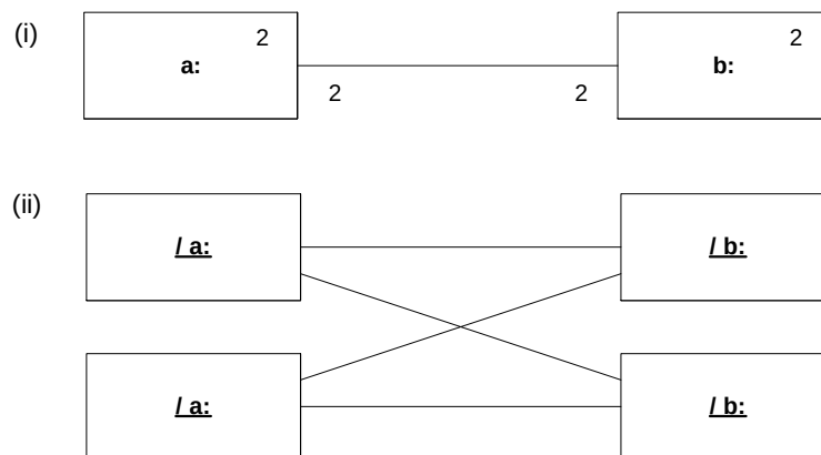
Figure 116 - “Star” connector pattern
