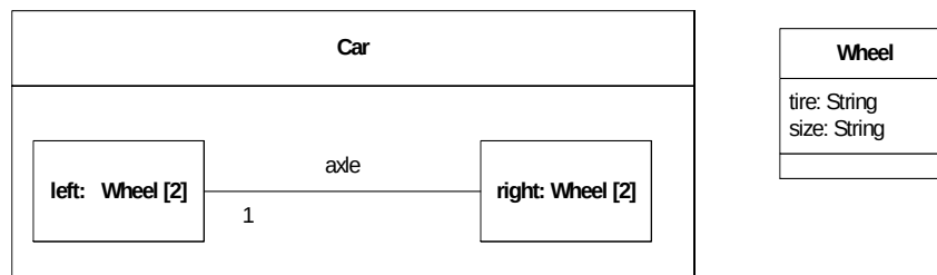
Figure 119 - Connectors and parts in a structure diagram using multiplicities
