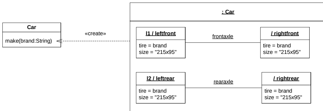
Figure 121 - A constructor for the Car class
