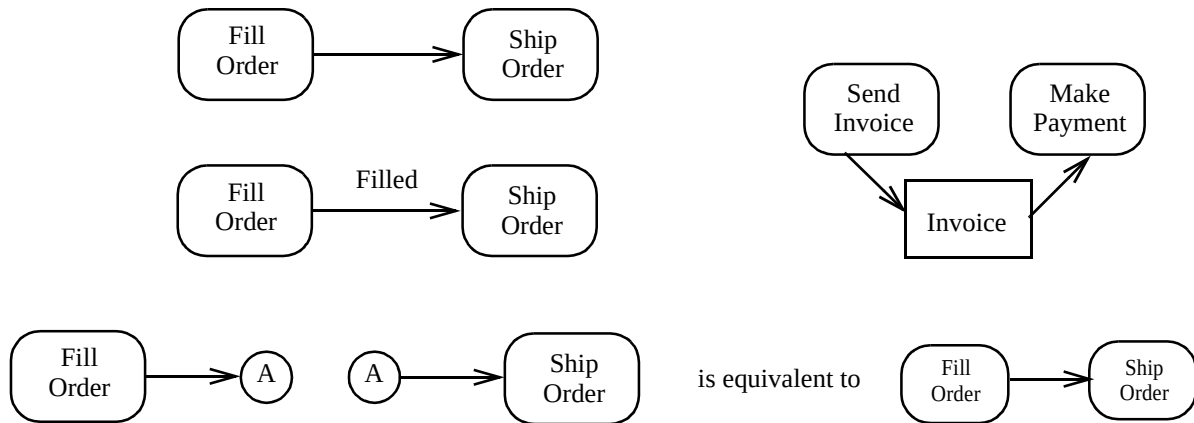
Figure 210 - Activity edge examples
