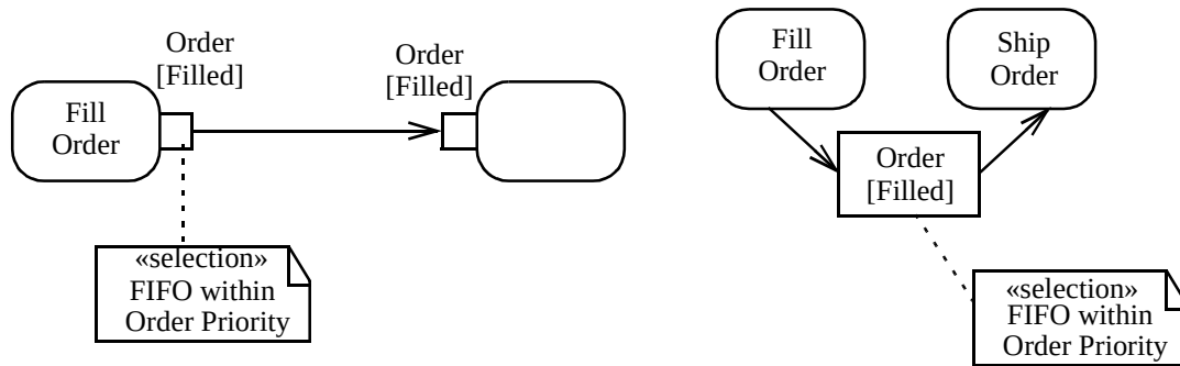
Figure 290 - Specifying selection behavior on an Object flow
