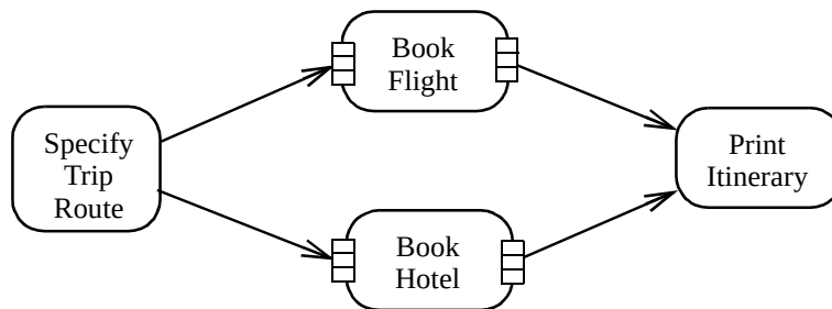
Figure 248 -Examples of expansion region shorthand
