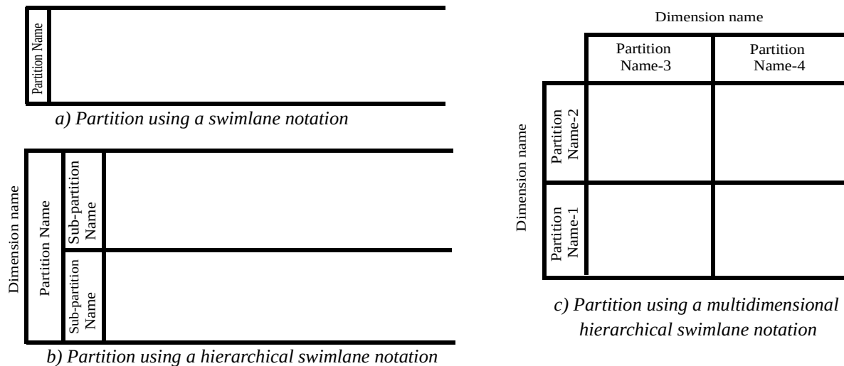
Figure 224 - Activity partition notations
