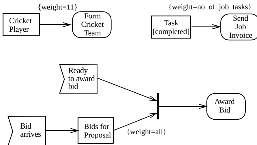
Figure 213 - Activity edge examples
