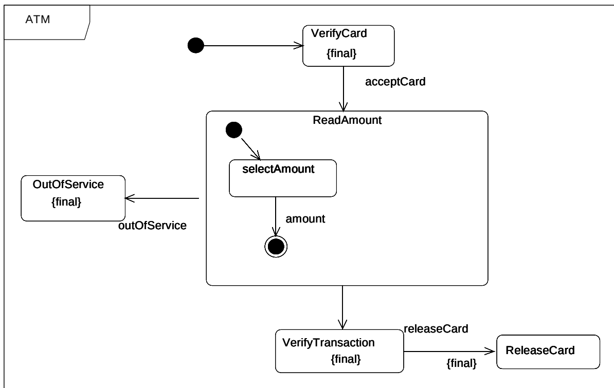
Figure 393 - A general state machine
