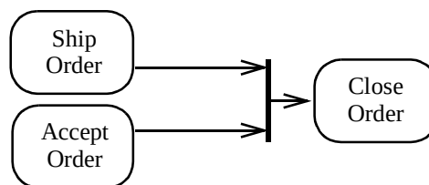
Figure 263 - Join node example
