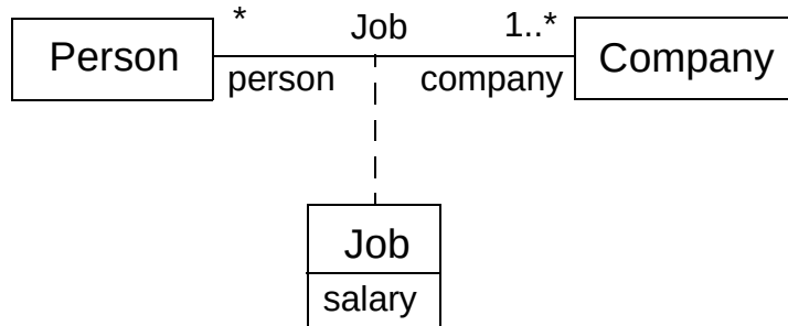
Figure 67 - An AssociationClass is depicted by an association symbol (a line) and a class symbol (a box) connected with a dashed line. The diagram shows the association class Job which is defined between the two classes Person and Company.
