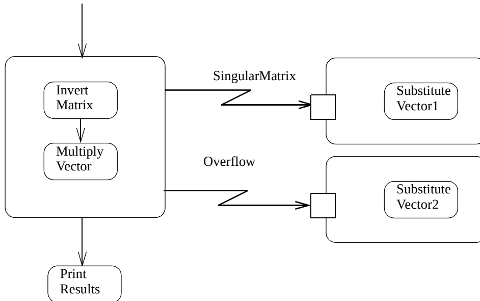
Figure 241 - Exception Handler example
