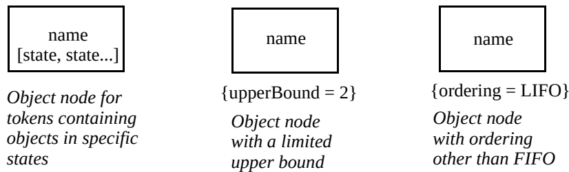
Figure 276 - Object node notations
