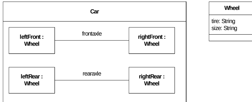
Figure 118 - Connectors and parts in a structure diagram
