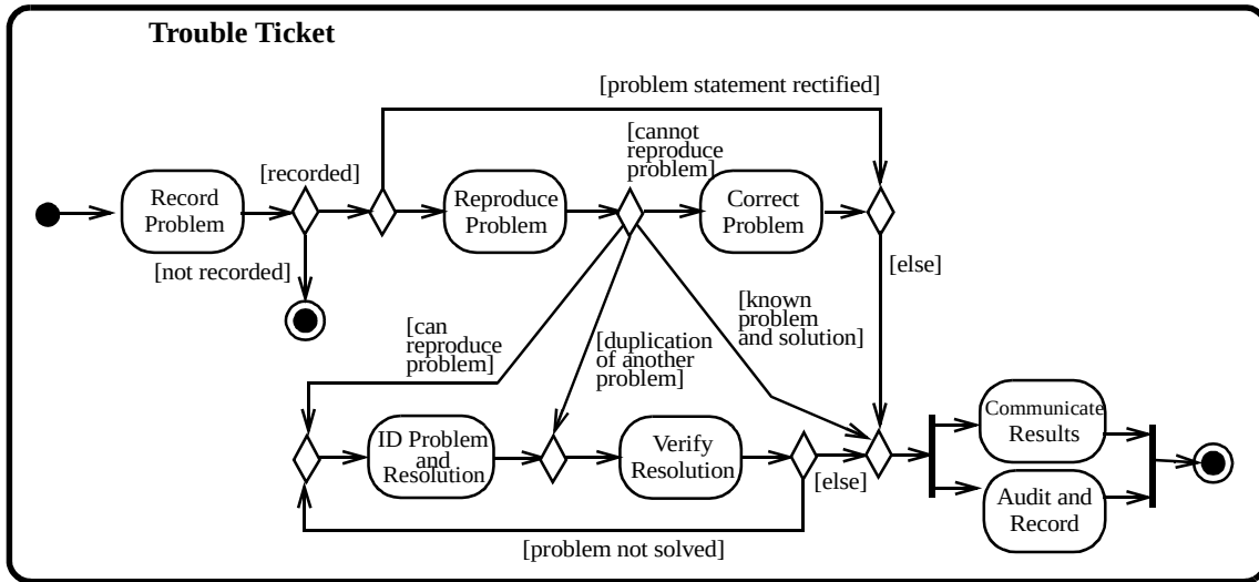
Figure 205 - Workflow based on example from the Workflow Process Definition RFP.
