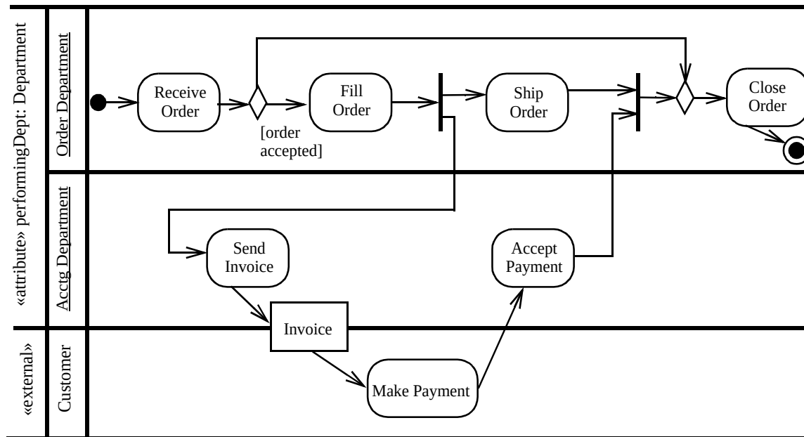
Figure 226 - Activity partition using swimlane example
