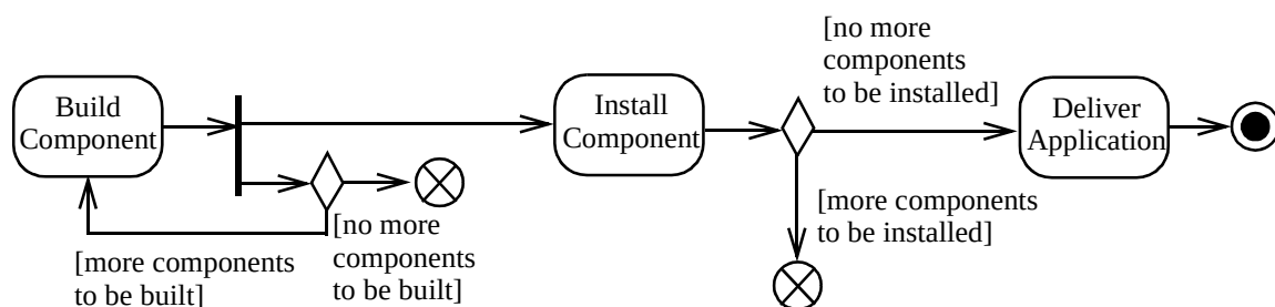
Figure 251 - Final node example.
