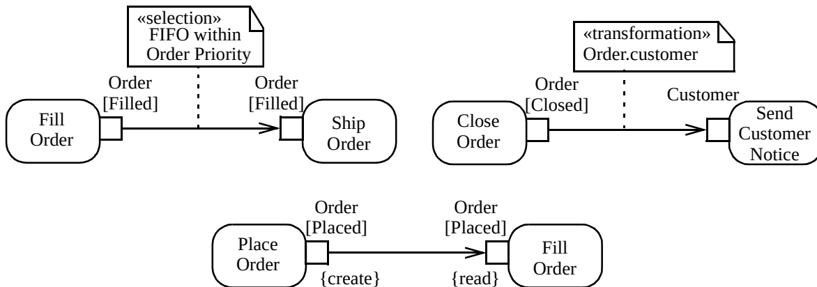
Figure 273 - Specifying selection behavior on an Object flow
