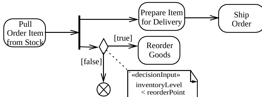
Figure 239 - Decision node example
