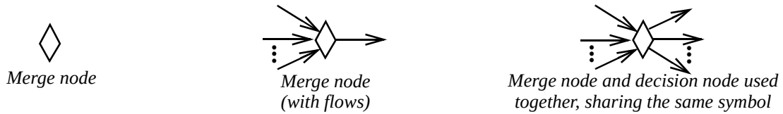
Figure 265 - Merge node notation
