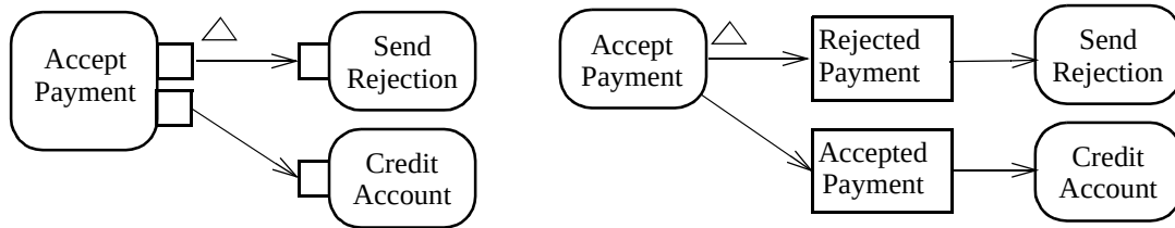
Figure 289 - Exception pin examples
