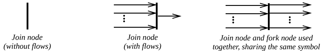
Figure 261 - Join node notations
