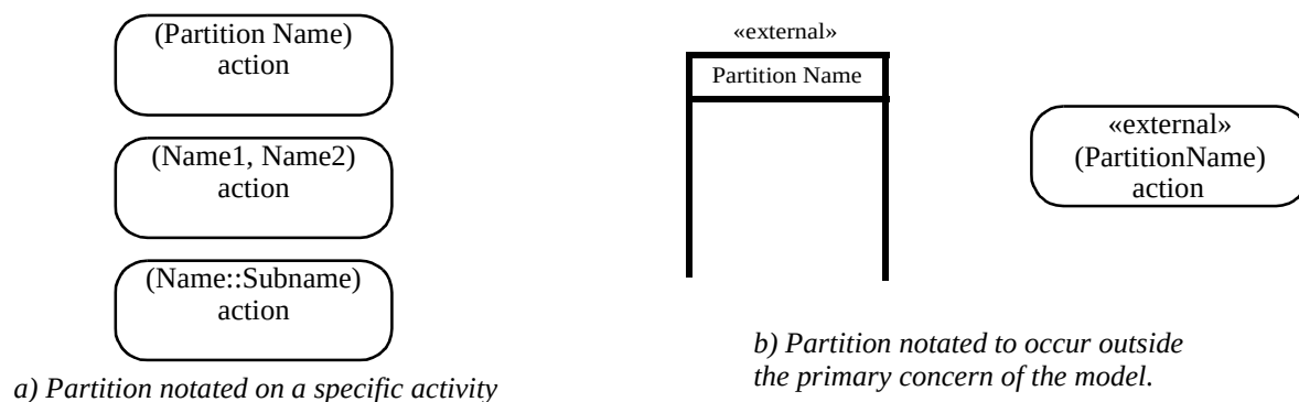
Figure 225 - Activity partition notations
