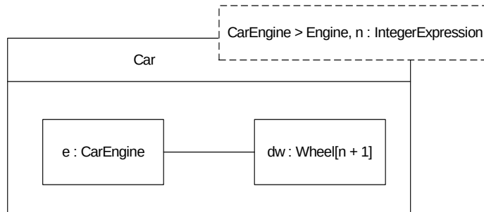
Figure 432 - Template Class with a constrained class parameter
