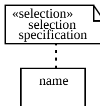
Figure 277 - Specifying selection behavior on an Object node
