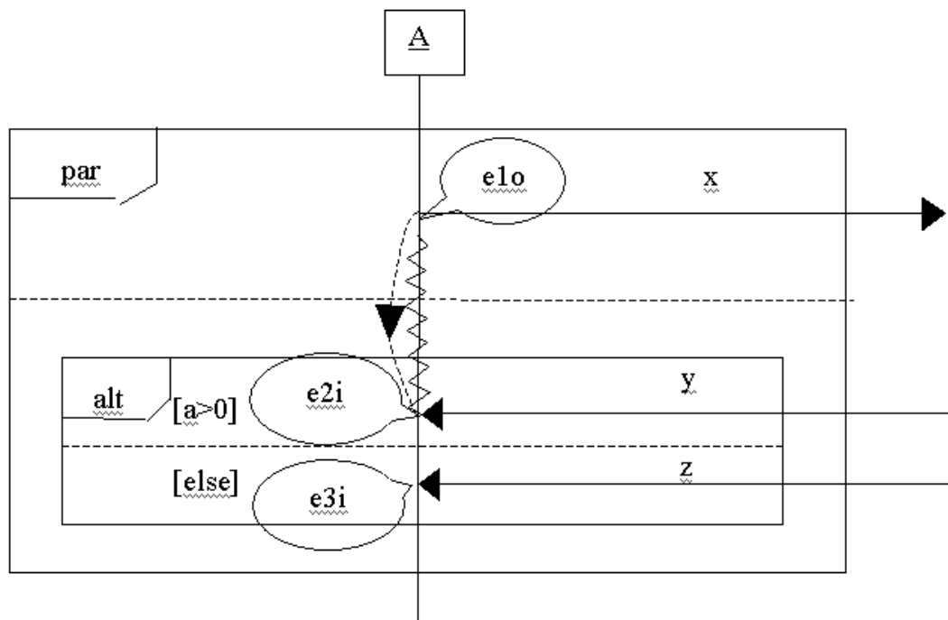
Figure 466 - Sequence diagram with guards, parallel composition and alternatives
