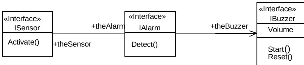
Figure 64 - A set of collaborating interfaces
