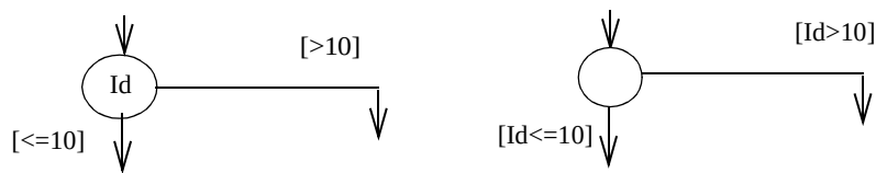
Figure 374 - Choice Pseudo State
