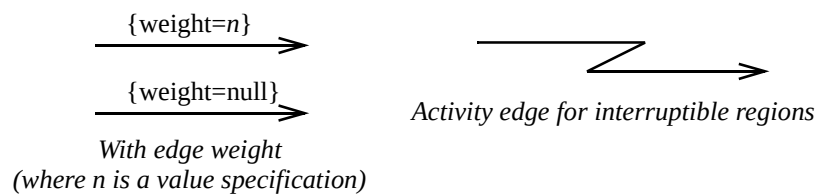
Figure 209 - Activity edge notation
