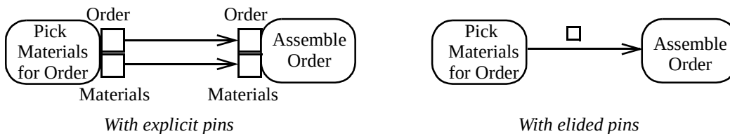
Figure 272 - Eliding objects flowing on the edge
