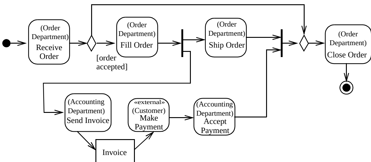
Figure 227 - Activity partition using annotation example
