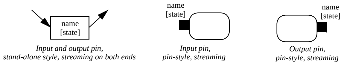
Figure 285 - Stream pin notations, with filled arrows and rectangles
