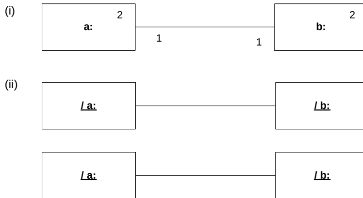
Figure 117 - “Array” connector pattern
