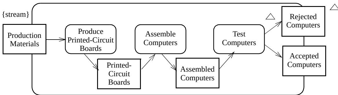
Figure 223 - Example of activity parameter nodes for streaming and exceptions
