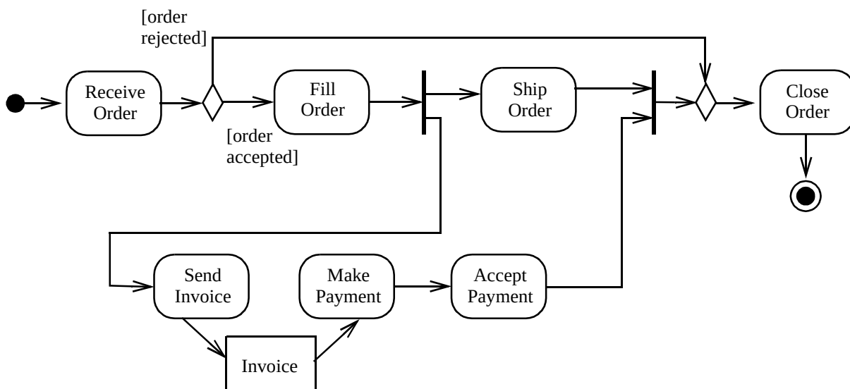
Figure 219 - Activity node example (where the arrowed lines are only the non-activity node symbols)
