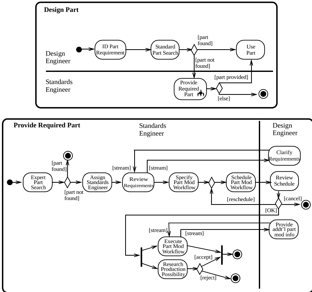
Figure 204 - Workflow based on example from the Workflow Process Definition RFP
