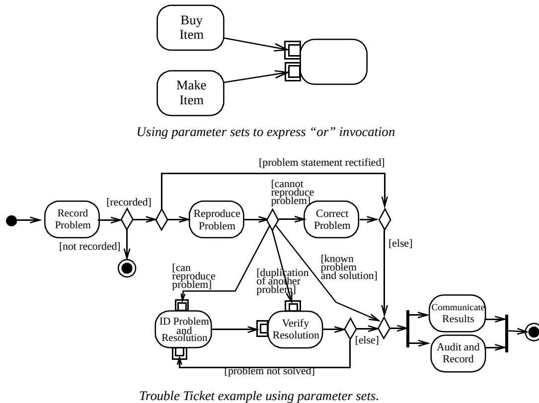
Figure 279 - Example of alternative input/outputs using parameter sets
