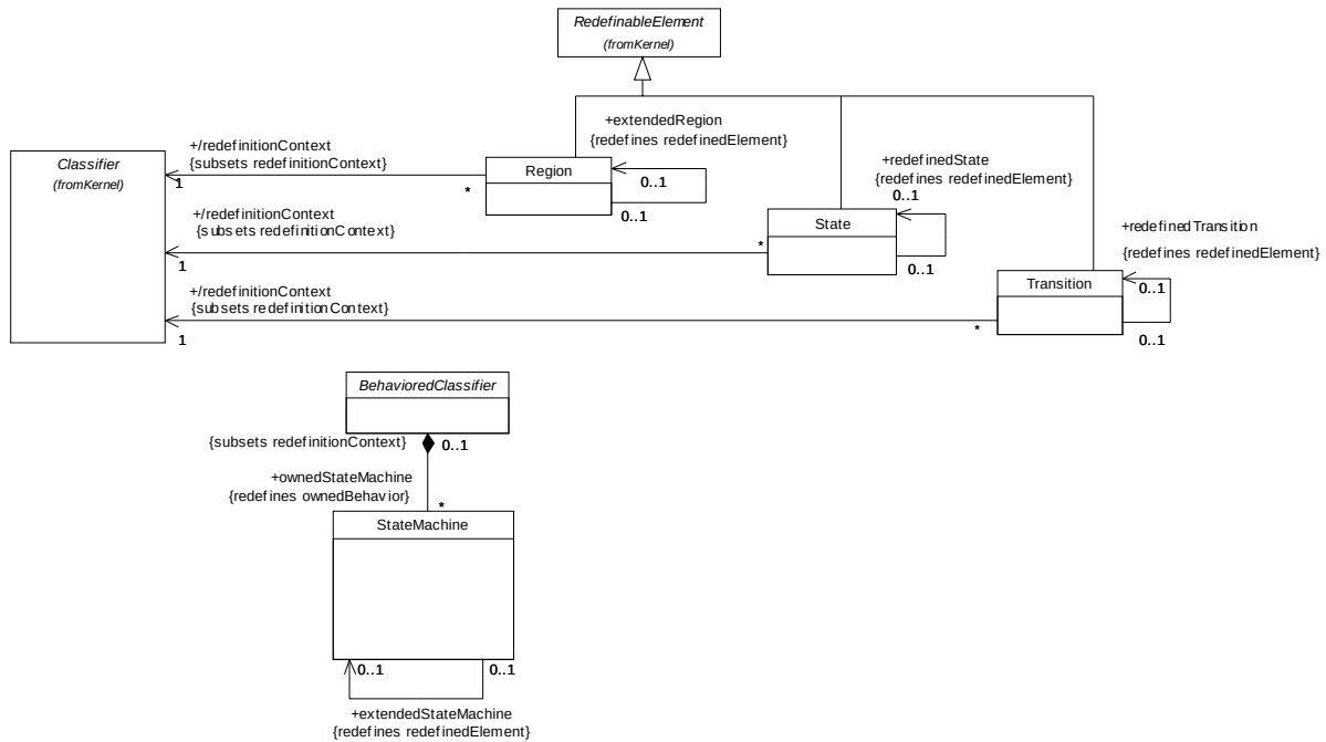
Figure 355 - State Machine Redefinitions
