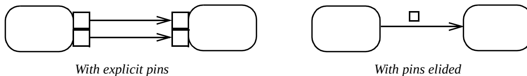
Figure 270 - Eliding objects flowing on the edge
