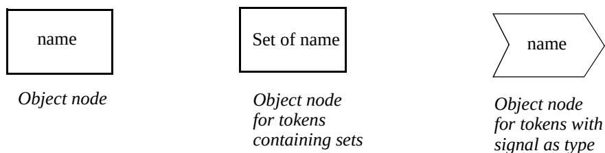
Figure 275 - Object node notations
