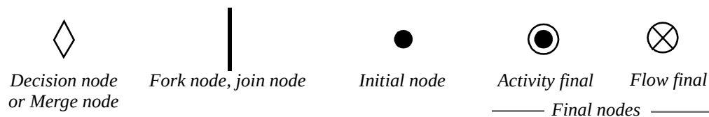
Figure 233 - Control node notations
