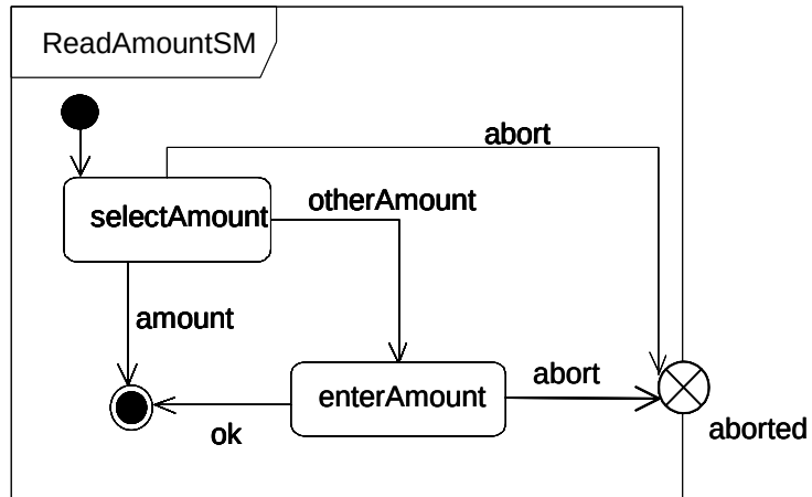
Figure 398 - State machine with exit point definition
