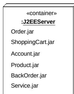
Figure 136 - Notation for a ExecutionEnvironment (example of an instance of a J2EE Server ExecutionEnvironment)
