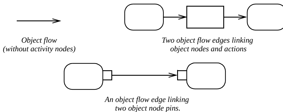
Figure 267 - Object flow notations
