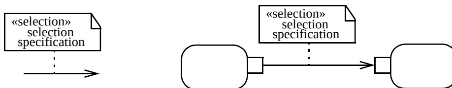
Figure 268 - Specifying selection behavior on an Object flow
