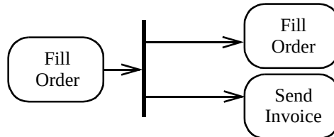
Figure 255 - Fork node example.
