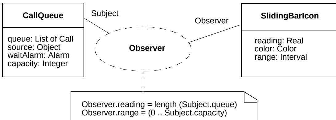
Figure 105 - In the Observer collaboration two roles, a Subject and an Observer, collaborate to produce the desired behavior. Any instance playing the Subject role must possess the properties specified by CallQueue, and similarly for the Observer role.
