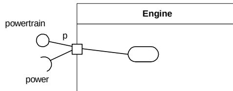
Figure 111 - Behavior port notation
