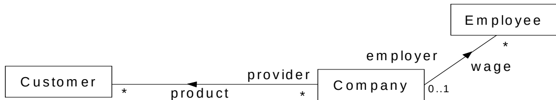
Figure 418 - Information Items attached to associations
