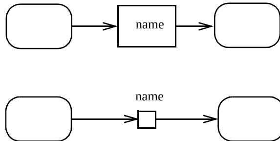
Figure 281 - Standalone pin notations
