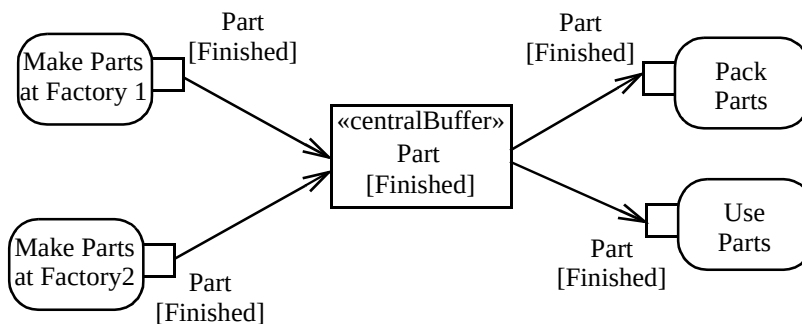
Figure 230 - Central buffer node example
