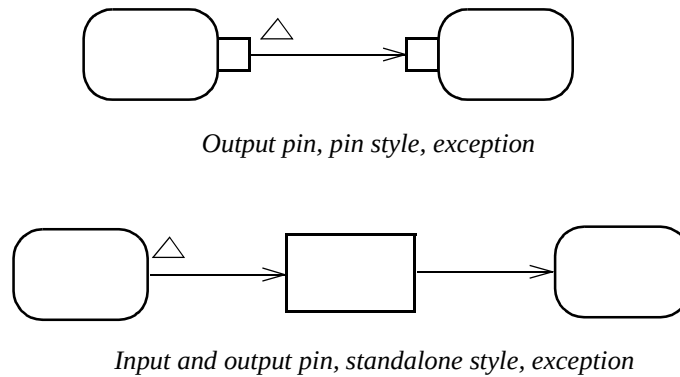
Figure 283 - Exception pin notations
