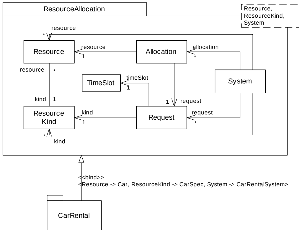
Figure 437 - Template Package and Bound Package
