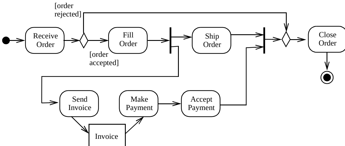
Figure 234 - Control node examples (with accompanying actions and control flows)
