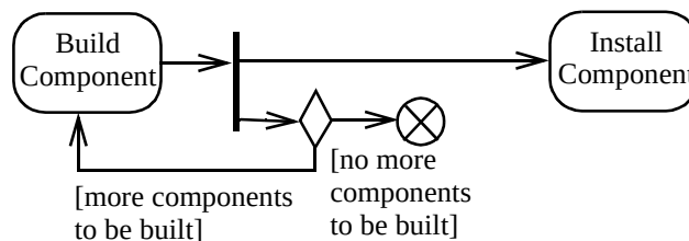
Figure 253 - Flow final example without merge edge
