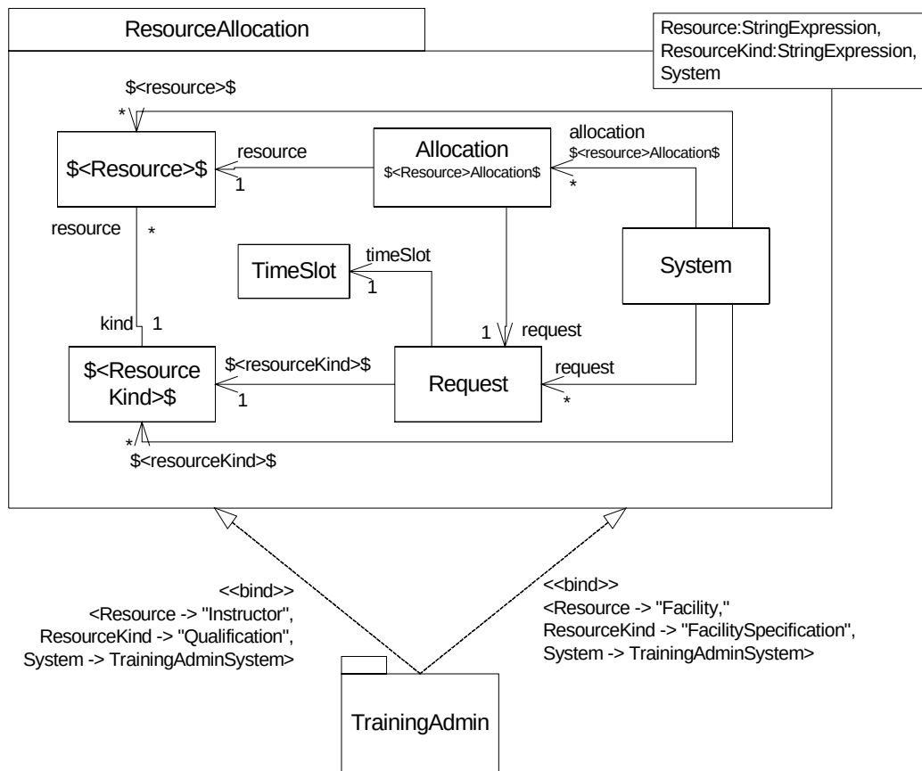
Figure 439 - Template Package with string parameters
