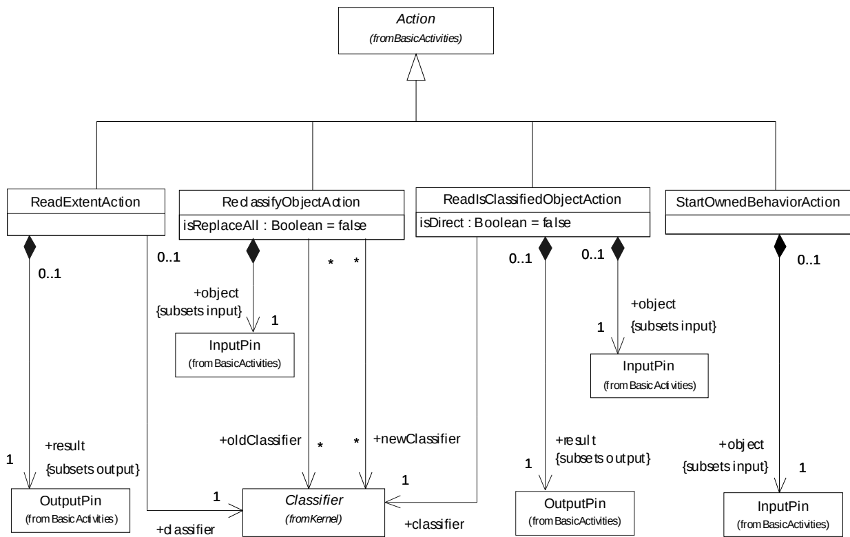
Figure 151 - Object actions (CompleteActions)
