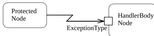
Figure 240 - Exception Handler Notation
