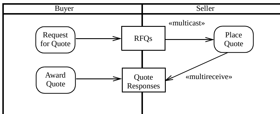
Figure 274 - Specifying multicast and multireceive on the edge
