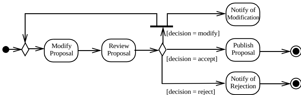
Figure 217 - Activity final example based on an example from the Workflow Process Definition RFP.
