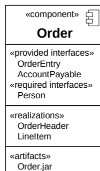
Figure 84 - A white-box representation of a component
