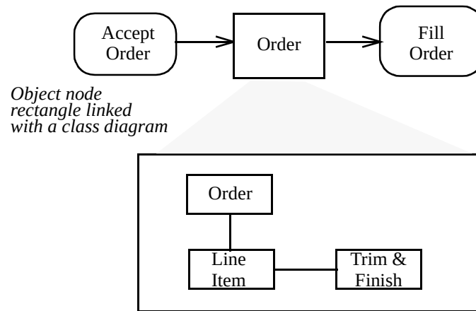
Figure 287 - Linking a class diagram to an object node
