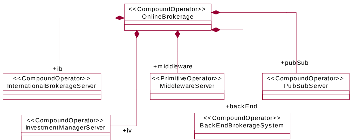
Figure 8-21 Class diagram for a compound operator with compound components
