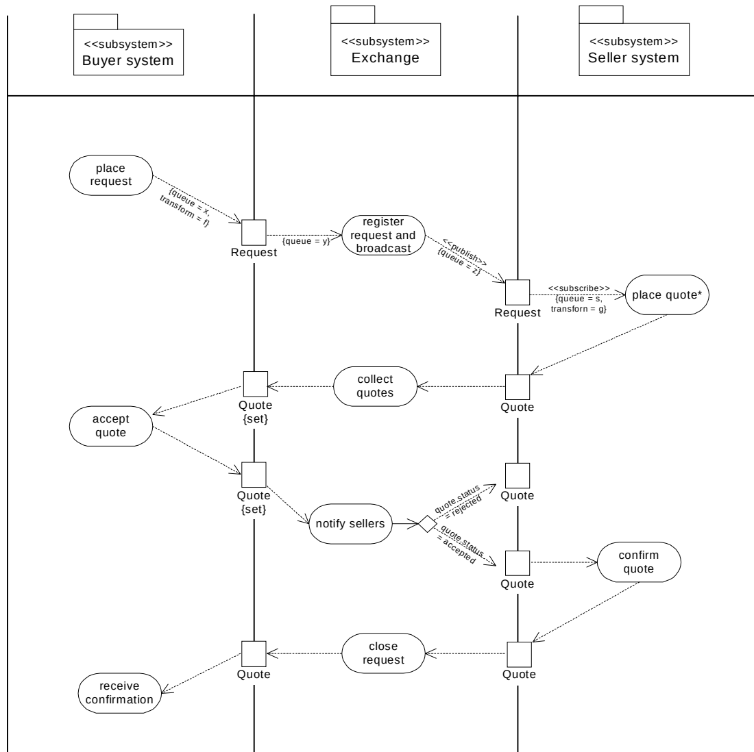
Figure 9-1 Basic way of modeling message based integration with Activities (Exchange example)
