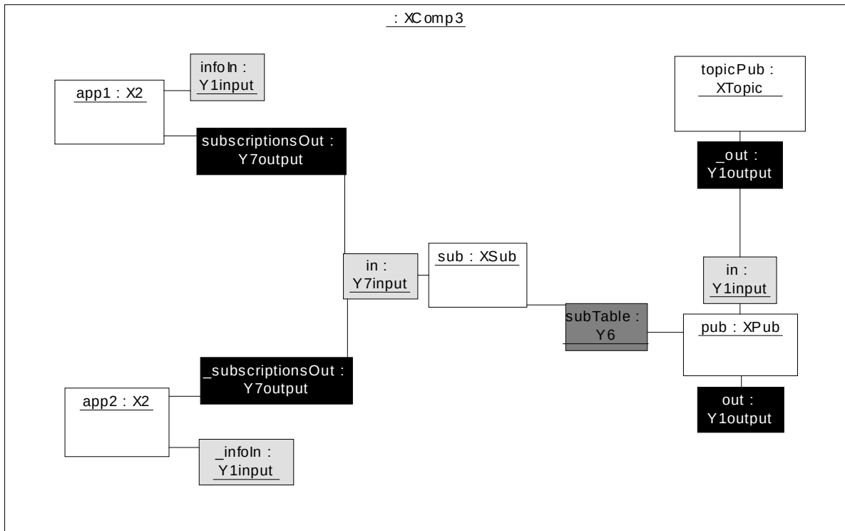
Figure 8-28 Configuration of publication and subscription operators
