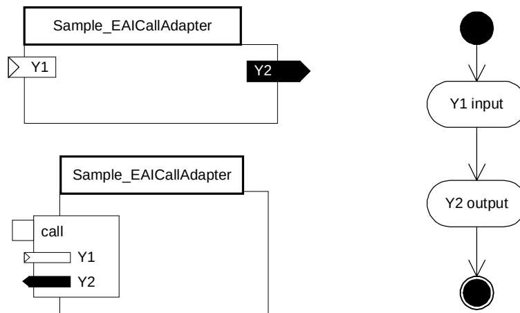
Figure 6-57 CCA notation for sample EAICallAdapter
