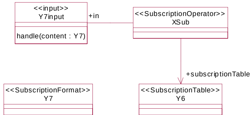
Figure 8-17 Class diagram for prototypical subscription operator
