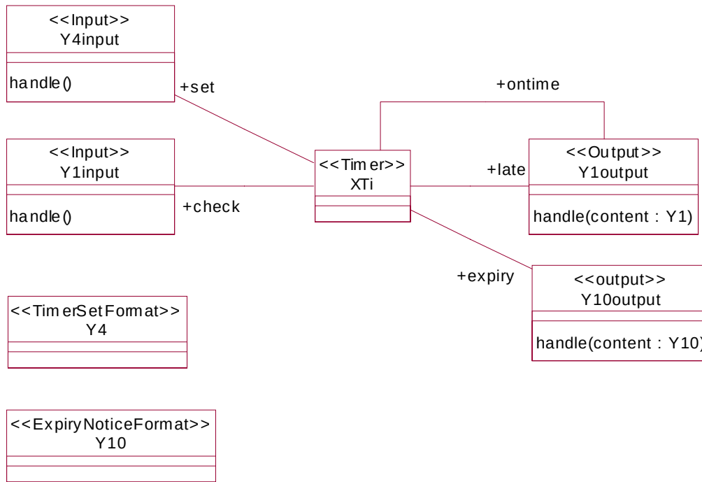
Figure 8-15 Class diagram for prototypical timer
