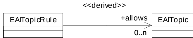
Figure 6-48 Relationship between publishers, subscribers and topics
