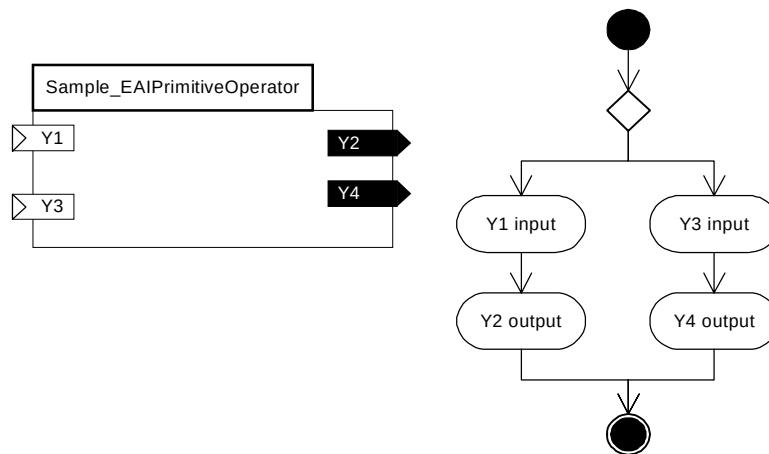
Figure 6-49 CCA notation for a sample generic EAIPrimitiveOperator
