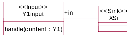
Figure 8-13 Class diagram for prototypical sink
