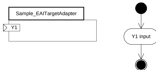
Figure 6-56 CCA notation for a sample EAITargetAdapter
