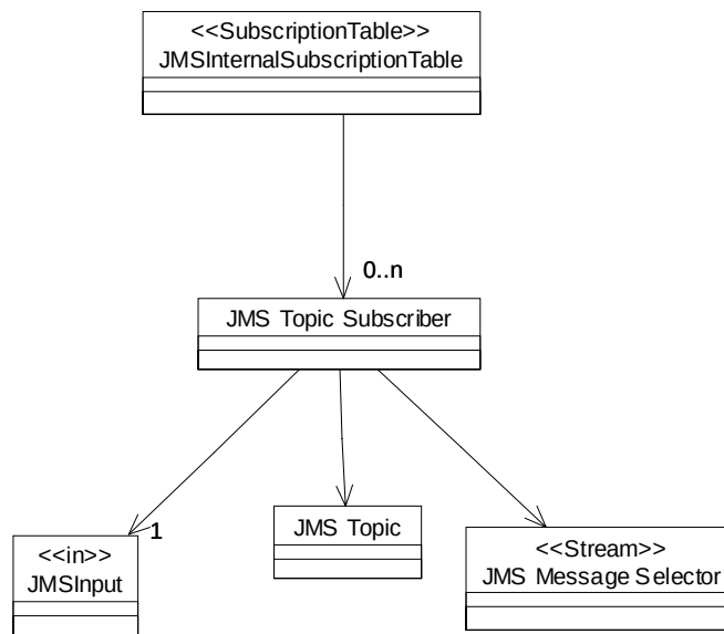
Figure 13-5 Model for the content of the JMS subscription table
