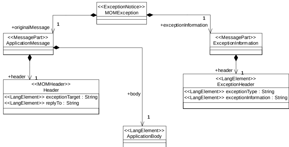
Figure 8-31 Example of the use of the ExceptionNotice and MOMHeader stereotypes
