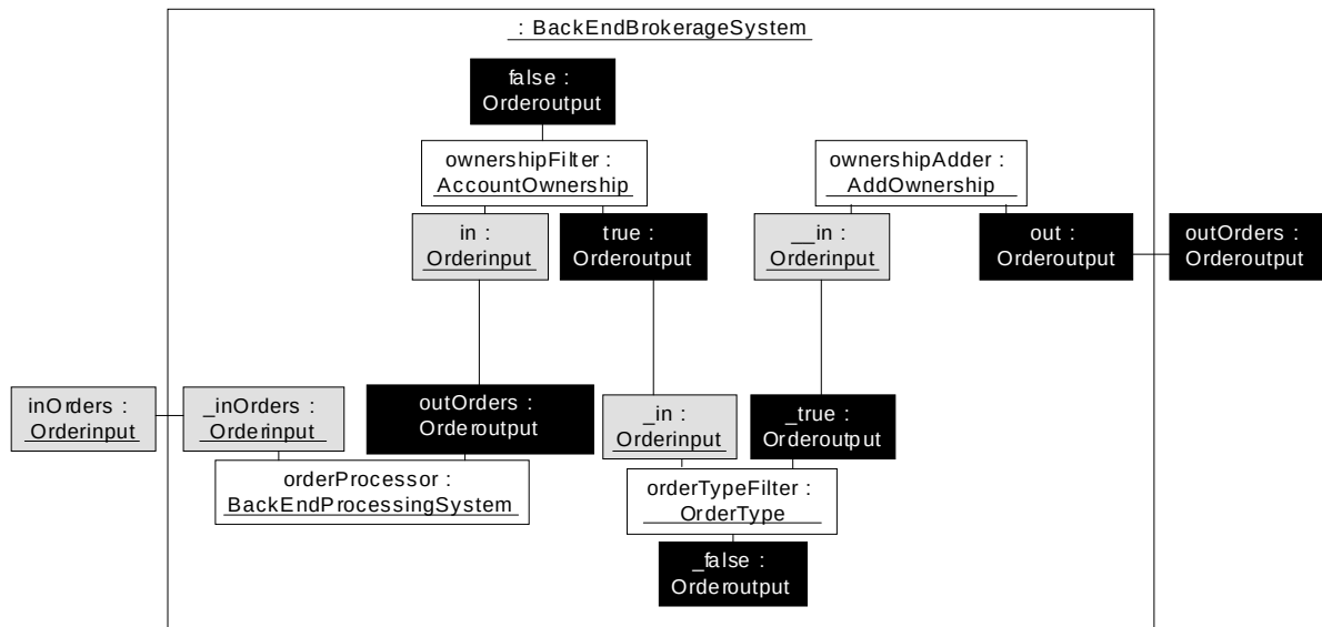
Figure 10-17 Back-end brokerage system - component connections
