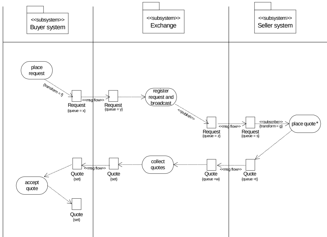
Figure 9-3 Application integration example with "messageflow" stereotype (partial)
