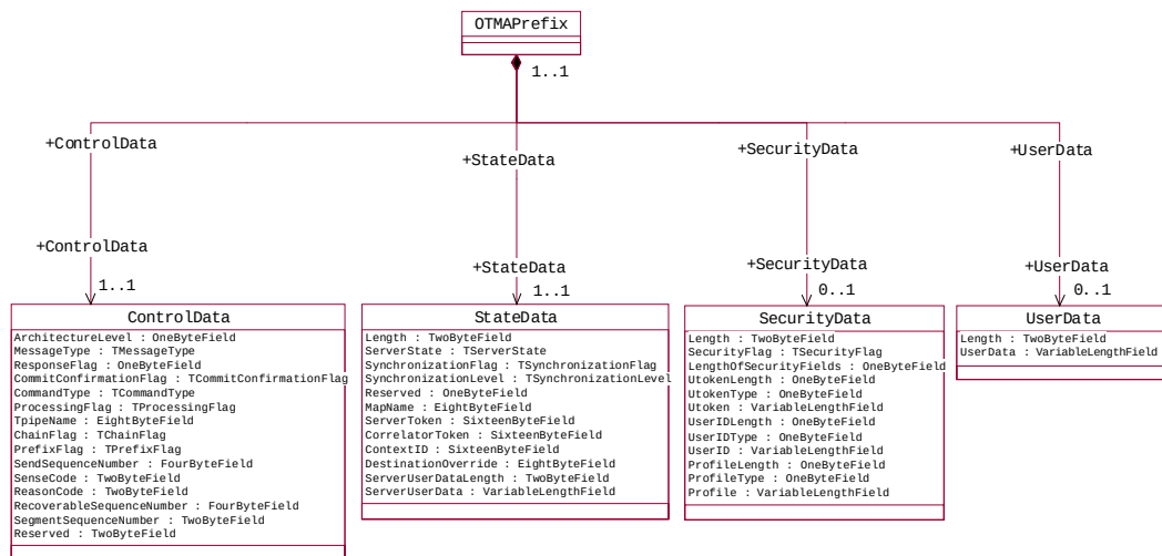
Figure A-2 IMS Transaction Message Prefix
