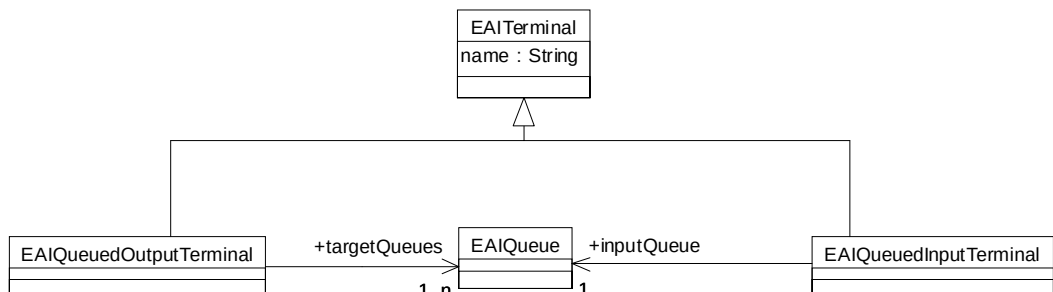
Figure 6-16 EAIQueuedOutputTerminal and EAIQueuedInputTerminal
