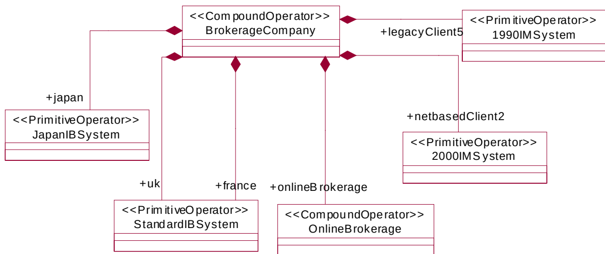
Figure 8-25 Class diagram for example with components of same type
