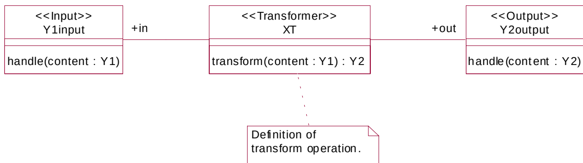
Figure 8-2 Class diagram for prototypical transformer
