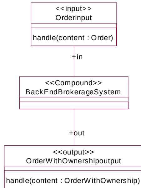
Figure 8-22 Terminals for example of compound operator
