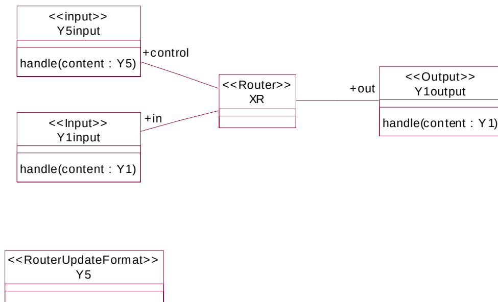
Figure 8-16 Class diagram for prototypical router
