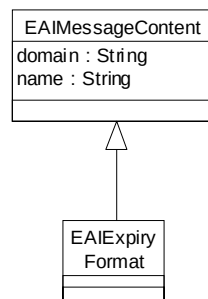
Figure 6-44 EAIDomainFormat
