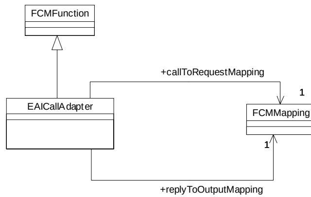
Figure 6-23 EAICallAdapter
