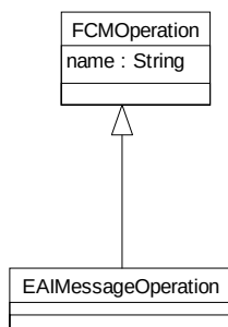
Figure 6-13 MessageOperation
