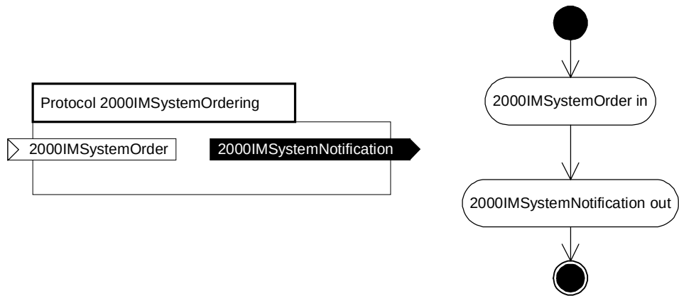
Figure 11-4 2000IMSystemOrdering Protocol
