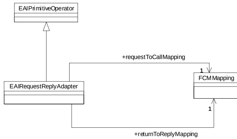
Figure 6-25 EAIRequestReplyAdapter
