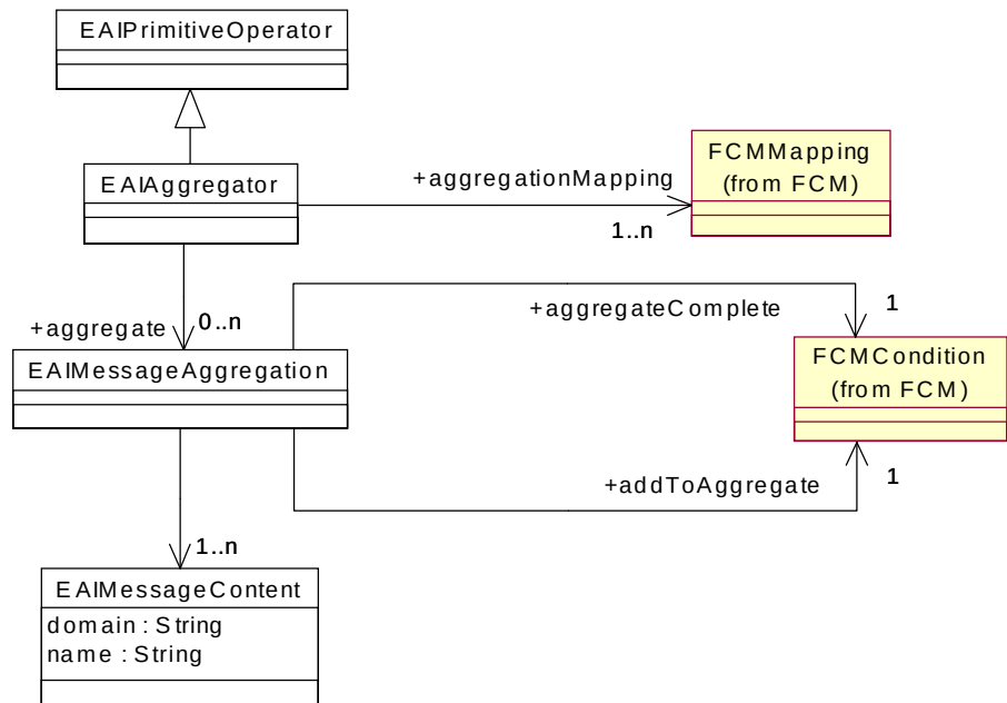
Figure 6-31 EAIAggregator
