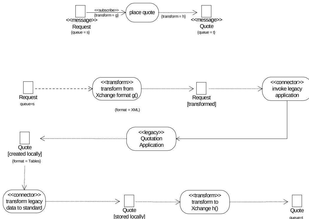
Figure 9-5 Decomposition of the integration step "Place Quote" in the context of the Exchange example
