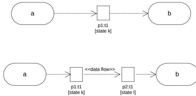
Figure 9-2 Application of the "messageFlow" stereotype to emphasize data-flow aspects
