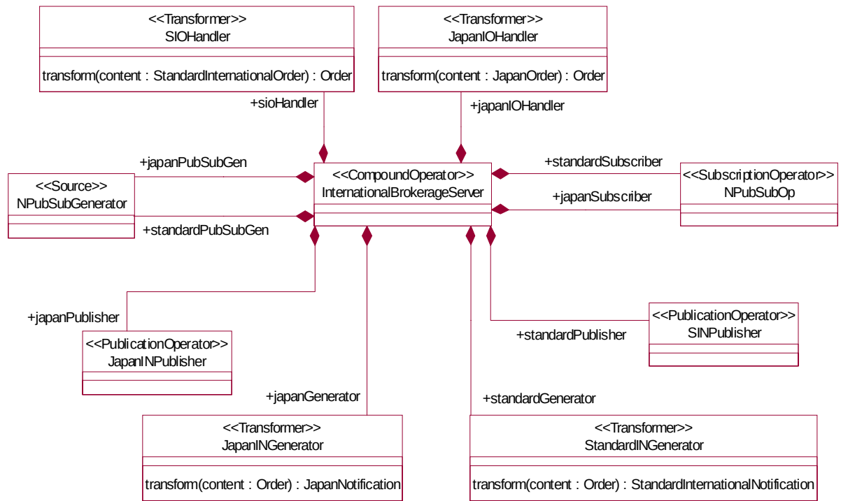
Figure 10-14 IBS - components
