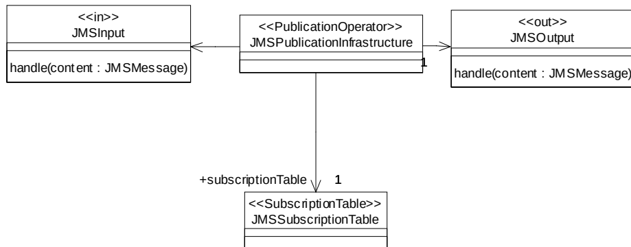
Figure 13-9 JMSPublicationInfrastructure
