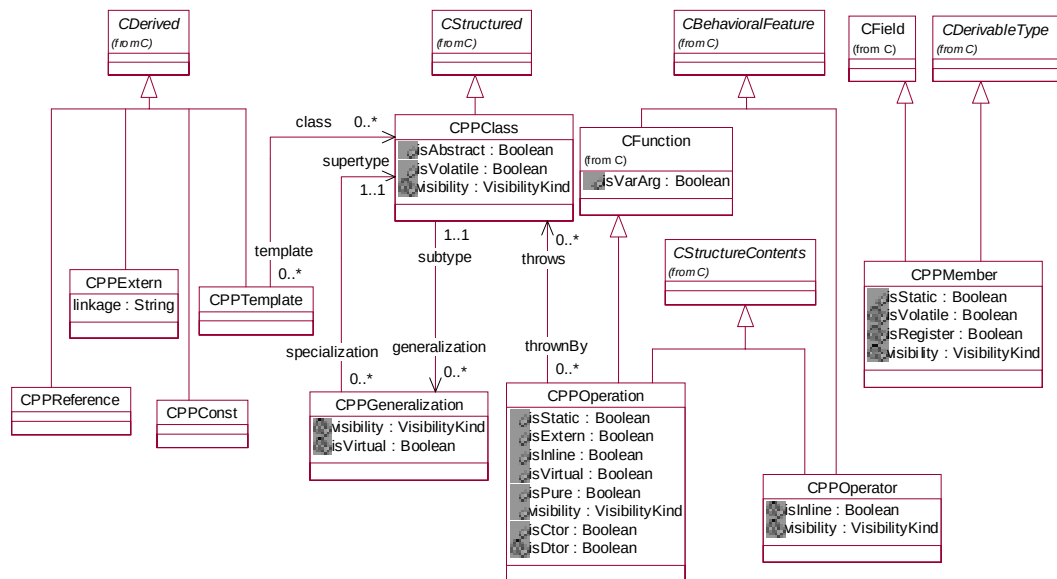
Figure 14-13 CPP Metamodel
