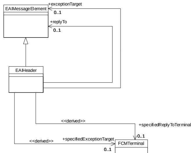
Figure 6-10 EAIHeader
