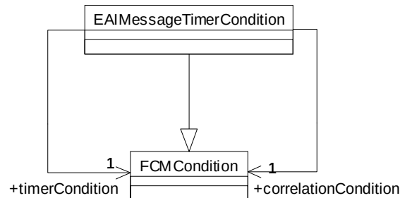
Figure 6-43 EAMessageTimerCondition
