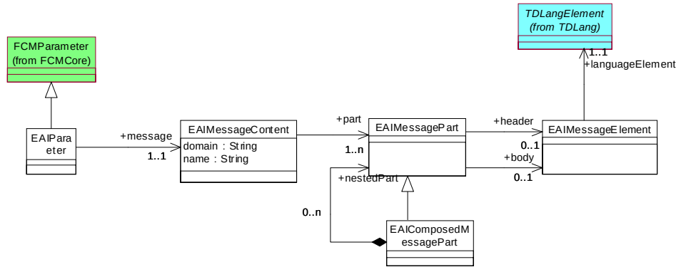
Figure 6-9 EAI MessageContent
