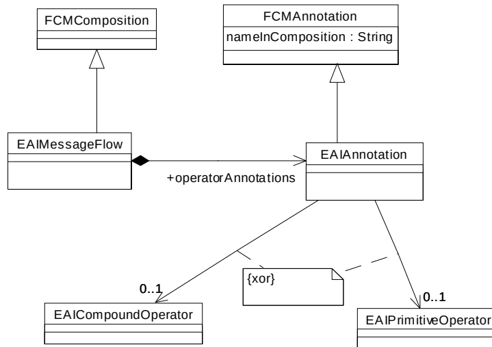
Figure 6-19 EAIMessageFlow
