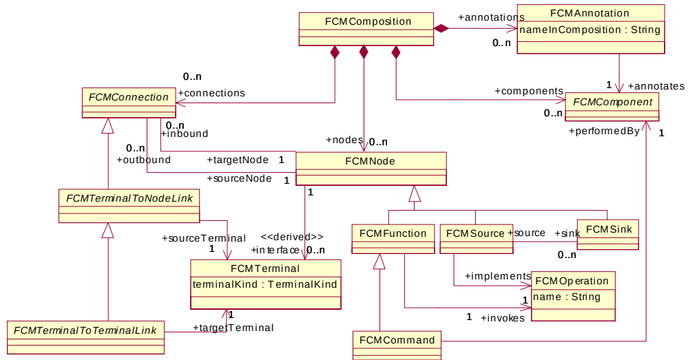
Figure 6-2 Flow Composition Model main diagram (from ad/2001-06-09)
