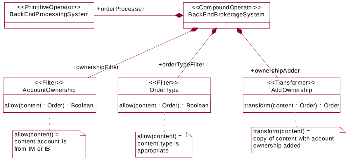
Figure 8-20 Class diagram for example compound operator
