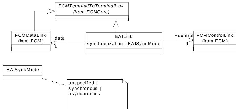
Figure 6-7 Definition of EAILink
