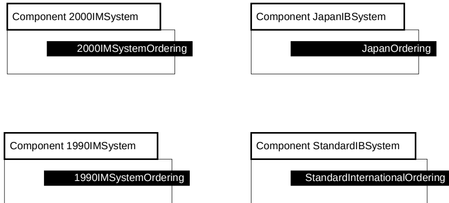
Figure 11-2 Ordering Components
