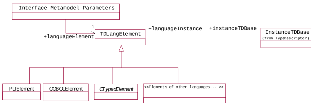
Figure 7-7 Convergent Metamodel
