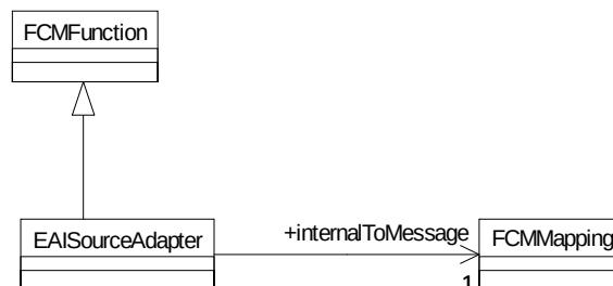
Figure 6-21 SourceAdapter
