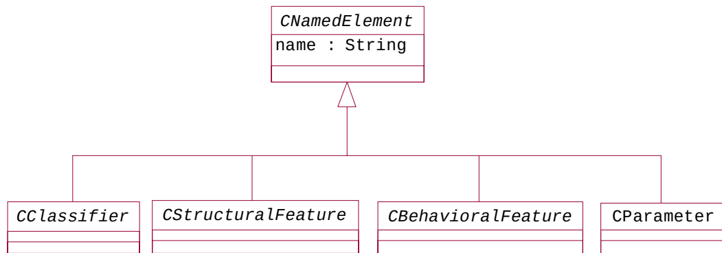
Figure 14-10 C Names
