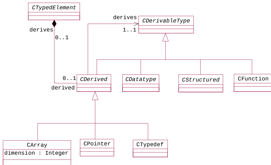
Figure 14-9 C Derivation
