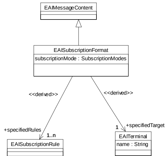
Figure 6-36 EAISubscriptionFormat
