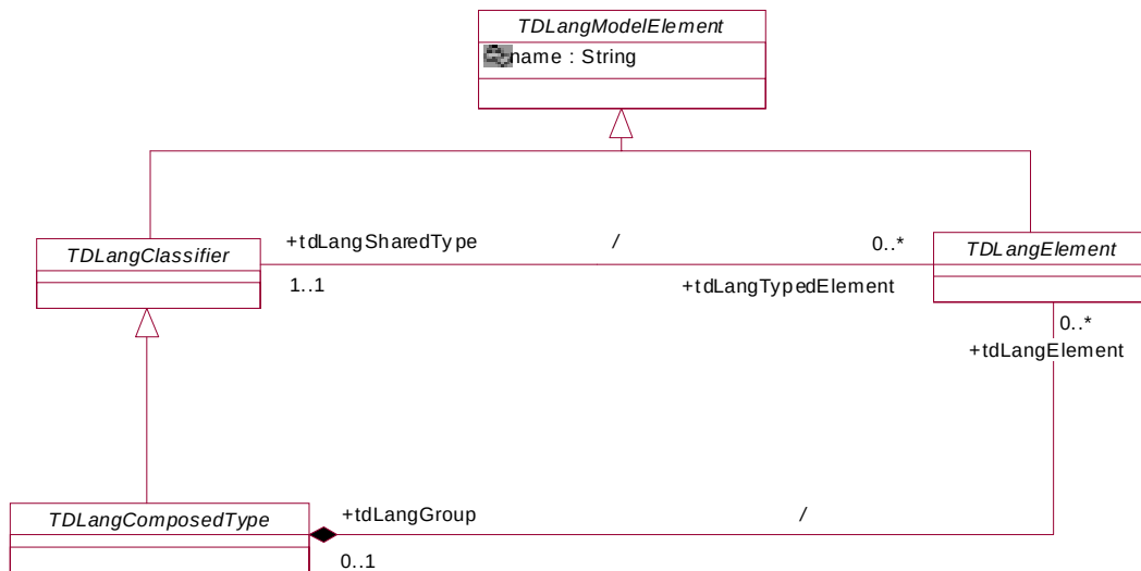
Figure 7-6 TDLang Metamodel
