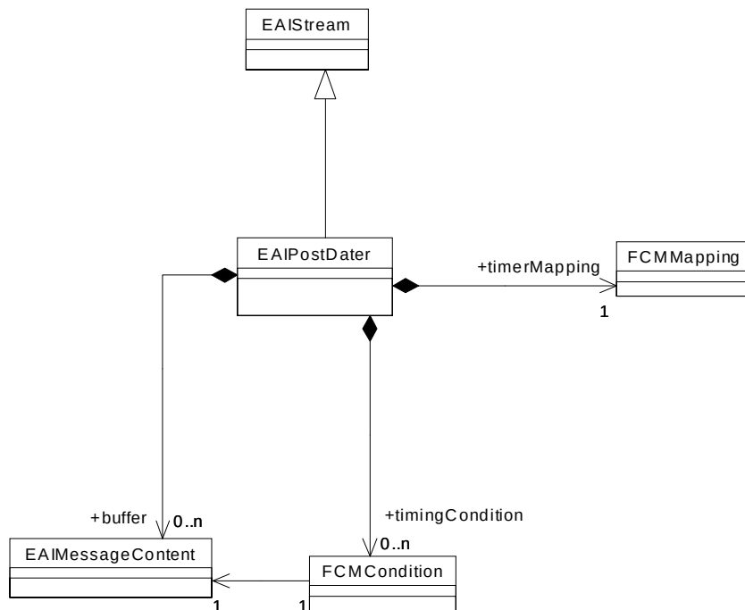
Figure 6-28 EAIPostDater
