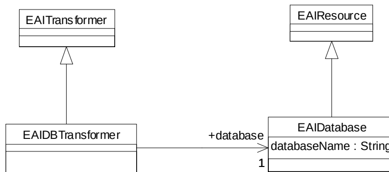
Figure 6-30 EAIDBTransformer
