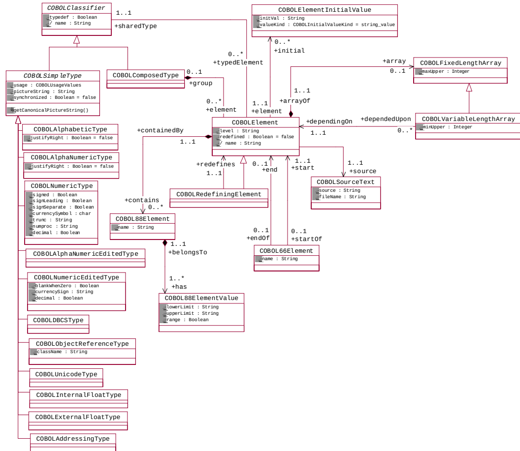
Figure 14-1 COBOL Metamodel
