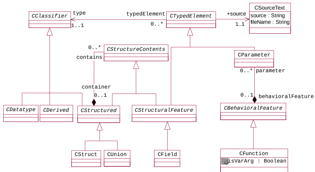
Figure 14-7 C Metamodel
