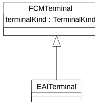
Figure 6-8 EAITerminal
