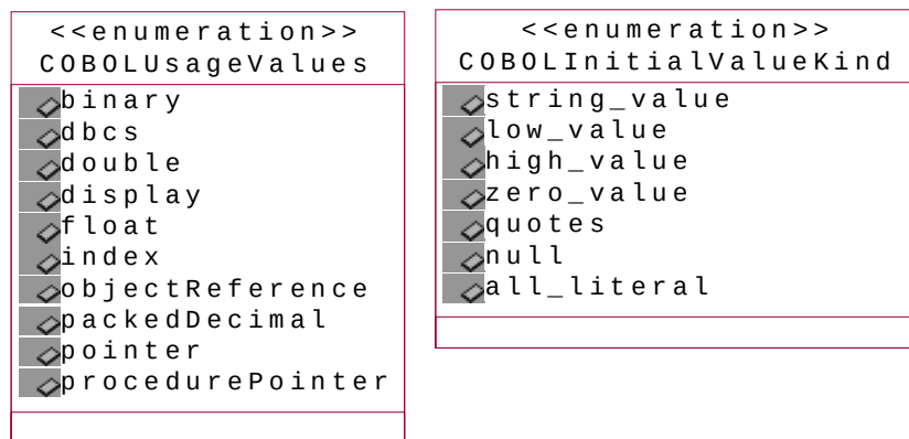
Figure 14-3 COBOL Stereotypes
