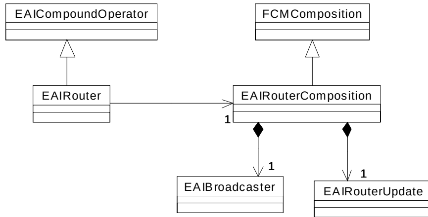
Figure 6-32 EAIRouter
