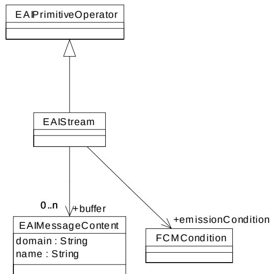
Figure 6-27 Stream
