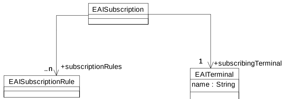
Figure 6-37 EAISubscription
