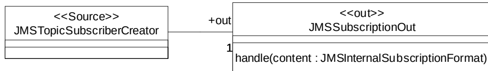
Figure 13-6 JMS TopicSubscriberCreator
