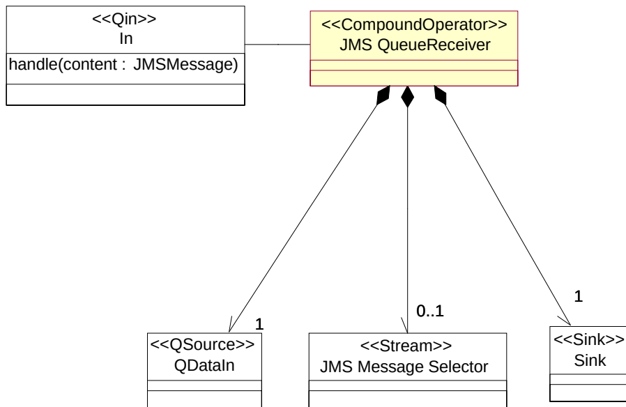
Figure 13-2 JMS QueueReceiver
