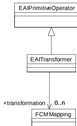
Figure 6-29 Transformer
