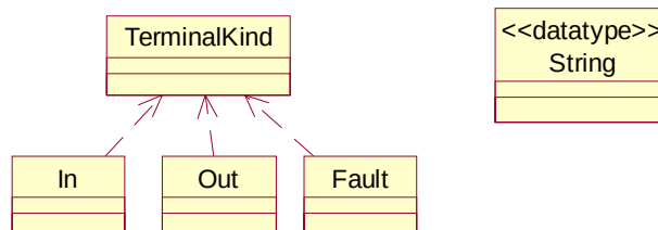
Figure 6-3 Flow Composition Model datatypes
