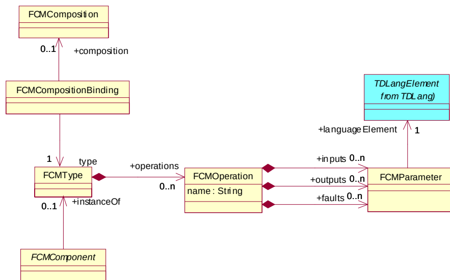
Figure 6-1 FCMComponent metamodel diagram (from ad/2001-06-09)
