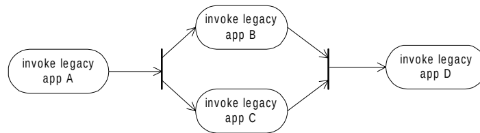
Figure 9-9 Synchronization with forks and joins
