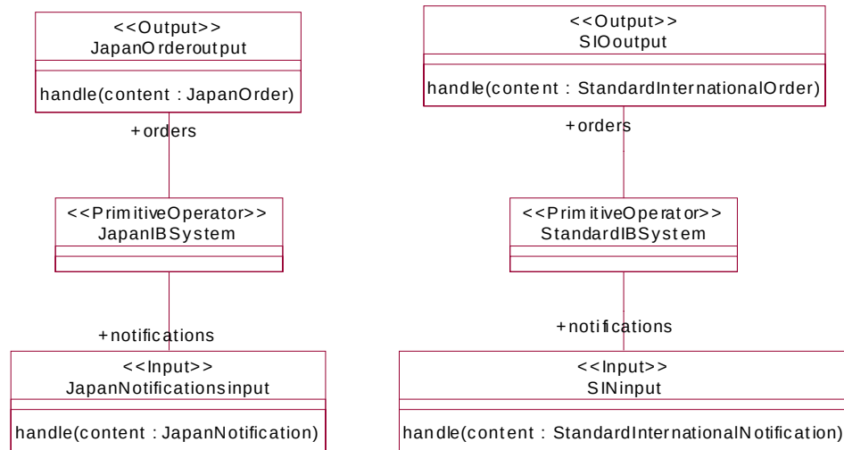
Figure 10-4 International brokerage systems - terminals
