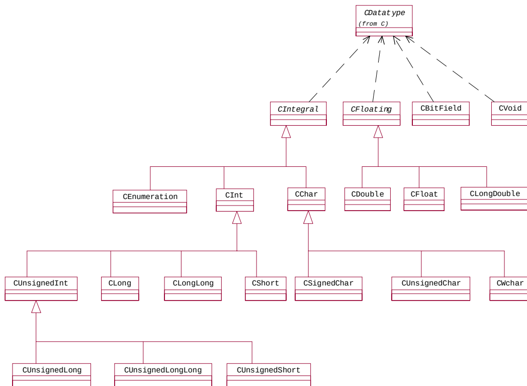
Figure 14-12 C User Types
