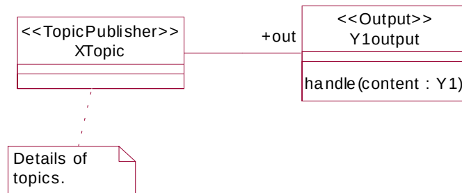
Figure 8-19 Class diagram for prototypical topic publisher
