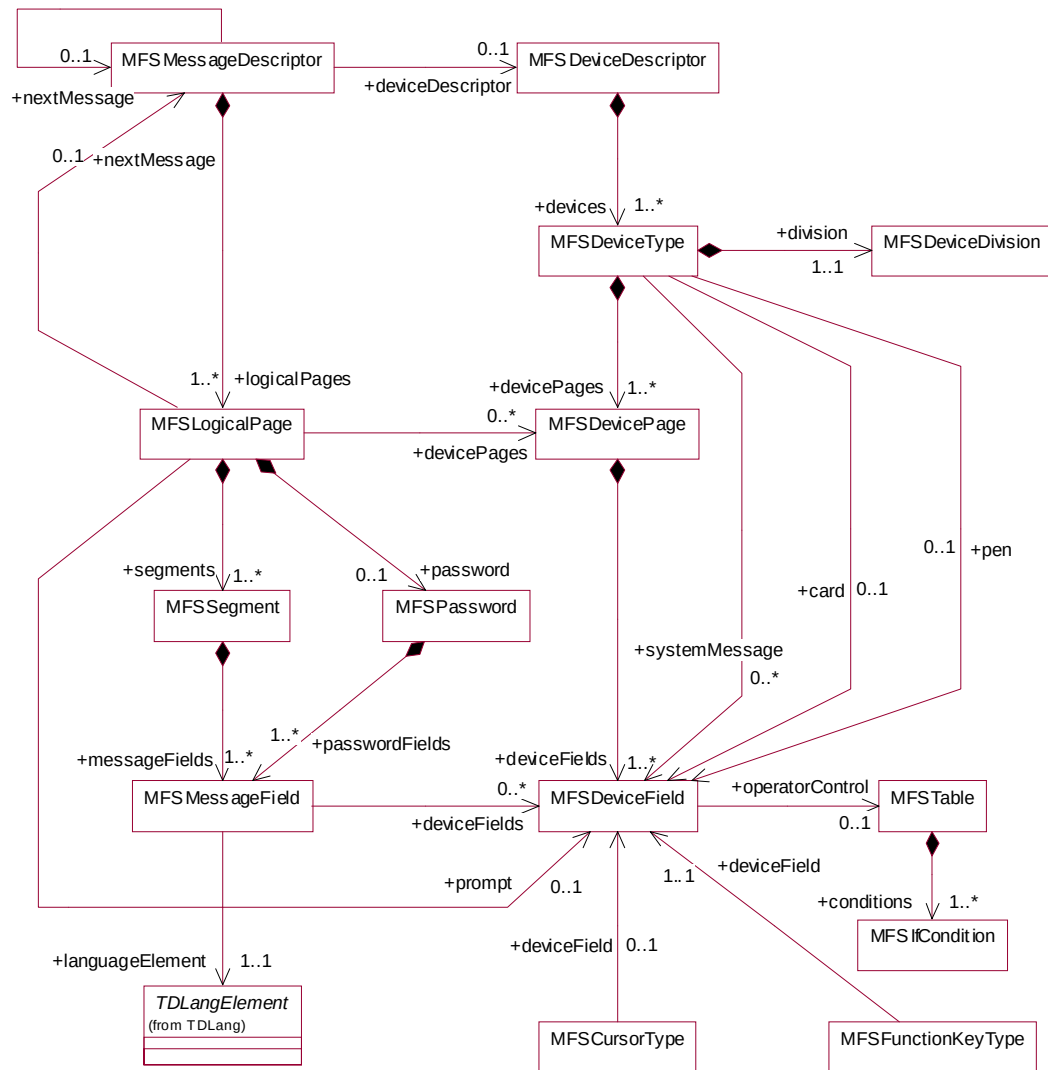
Figure A-8 MFS Relationship View
