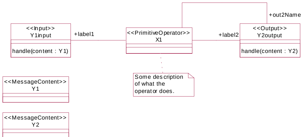
Figure 8-1 Class diagram for prototypical primitive operator with terminals
