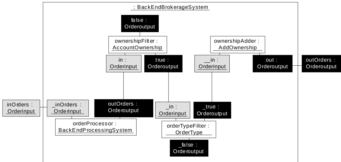
Figure 8-23 Collaboration diagram for example compound operator
