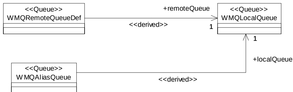
Figure 12-1 WMQRemoteQueue and WMQAliasQueue
