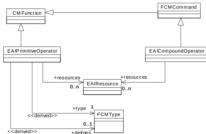
Figure 6-18 Definitions of PrimitiveOperator and CompoundOperator
