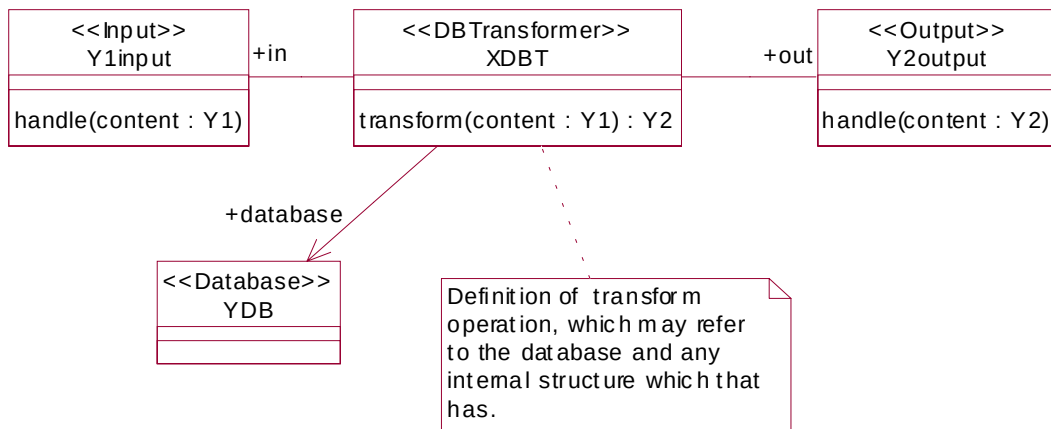
Figure 8-3 Class diagram for prototypical database transformer
