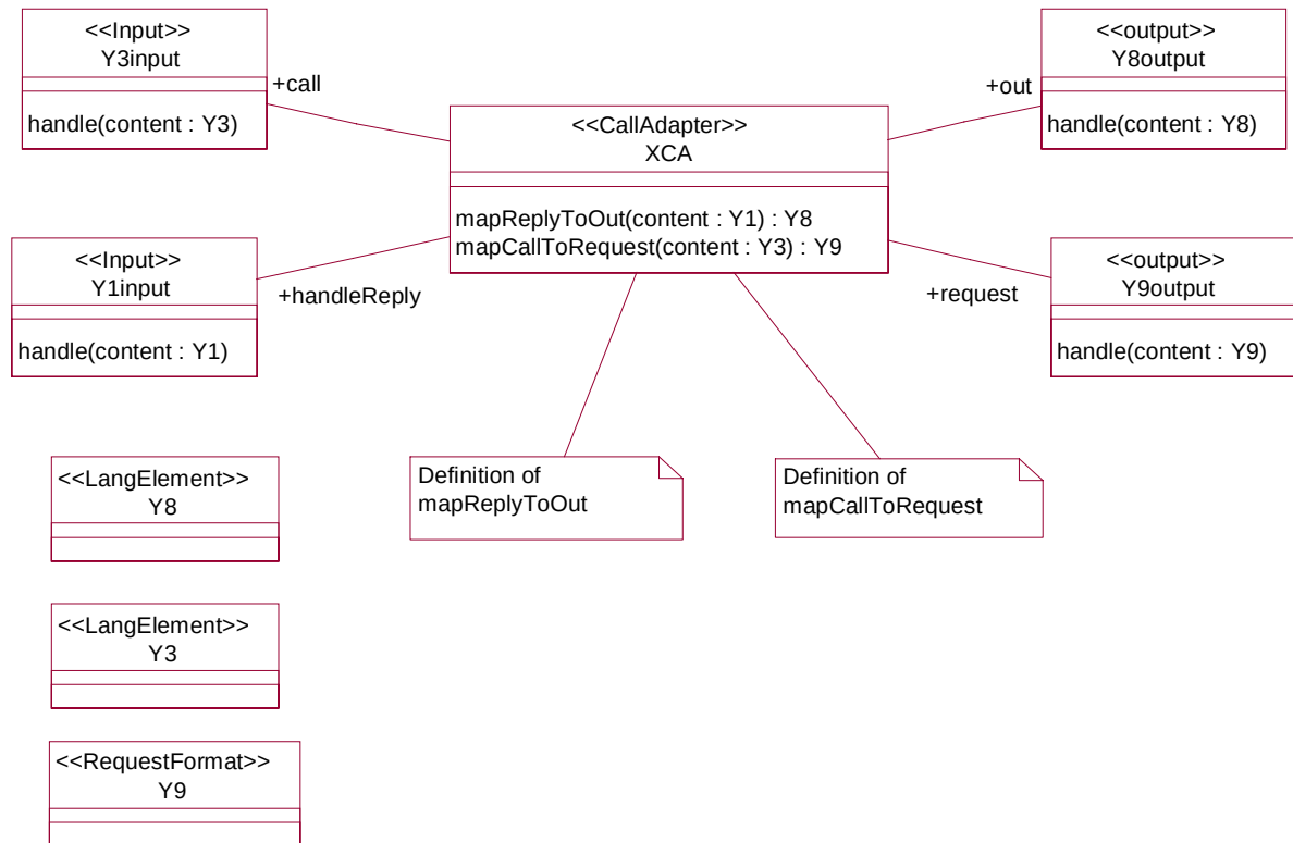
Figure 8-9 Class diagram for prototypical call adapter
