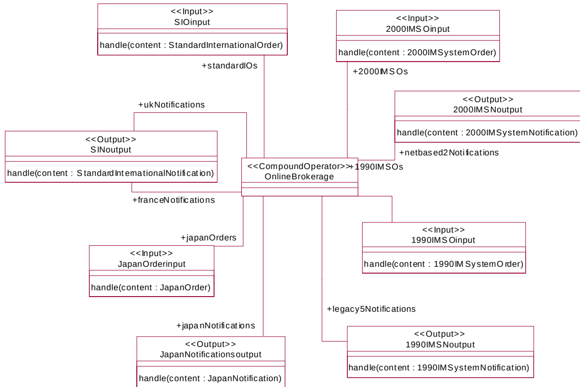
Figure 10-6 On-line brokerage system - terminals
