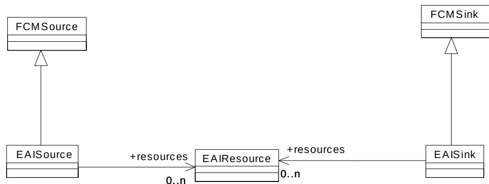
Figure 6-14 Sources and sinks
