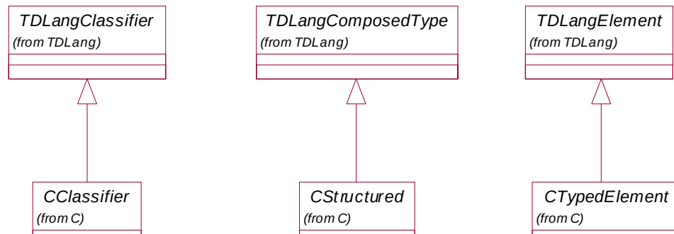
Figure 14-8 TDLang to C
