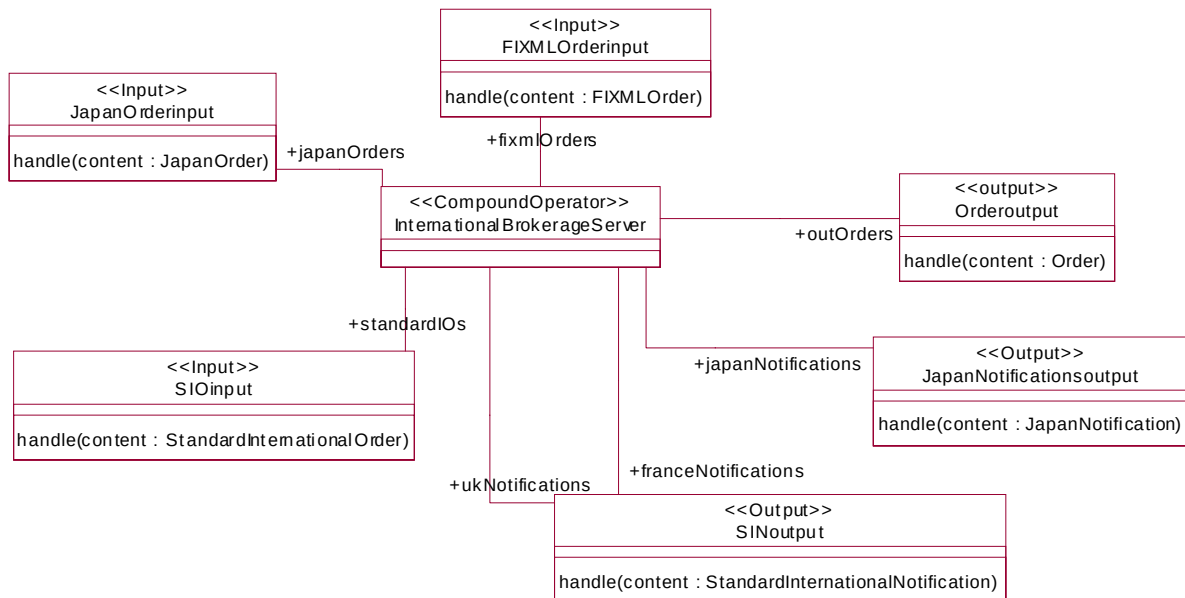
Figure 10-9 International brokerage server - terminals
