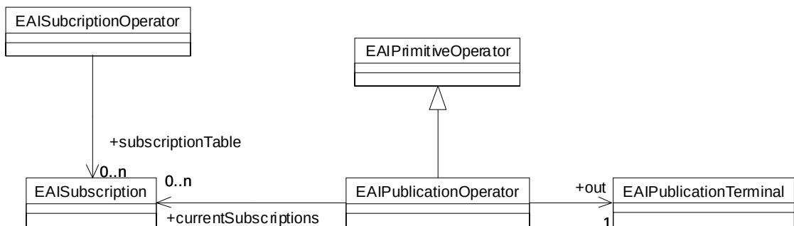
Figure 6-40 EAIPublicationOperator and EASubscriptionOperator
