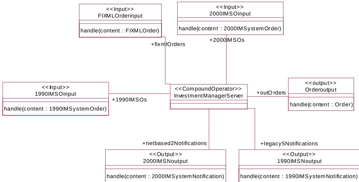
Figure 10-10 Investment-manager server - terminals
