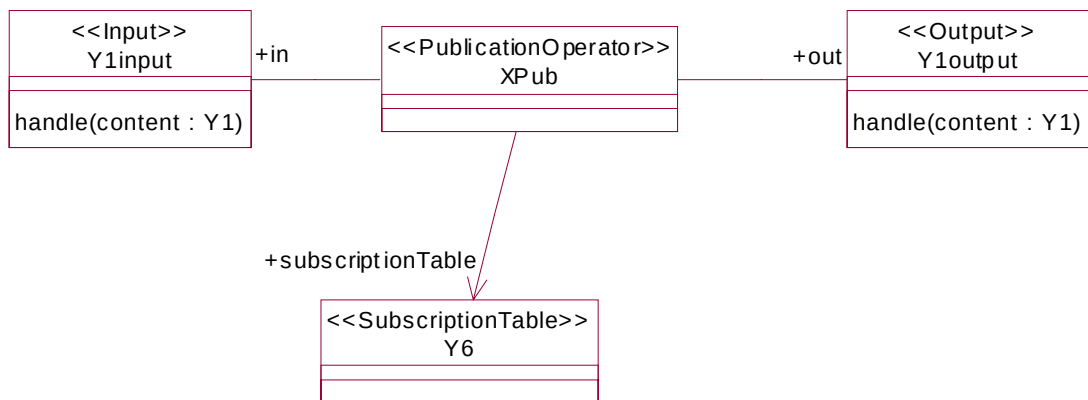
Figure 8-18 Class diagram for prototypical publication operator
