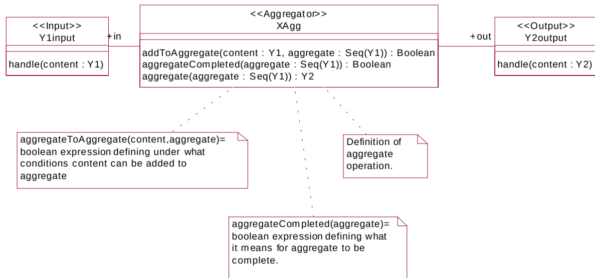
Figure 8-14 Class diagram for prototypical aggregator
