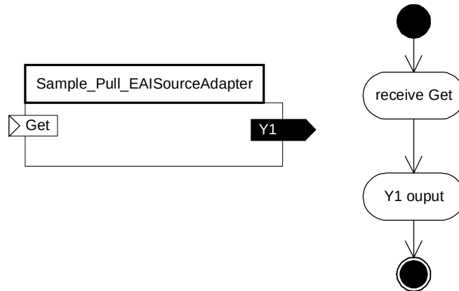
Figure 6-55 CCA notation for a sample Pull mode EAISourceAdapter
