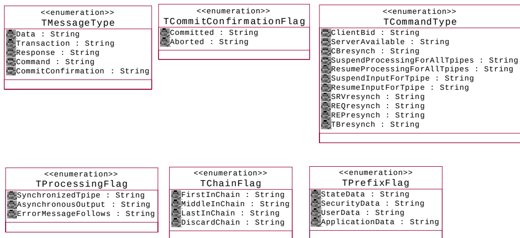
Figure A-3 OTMA Prefix - Defined Types
