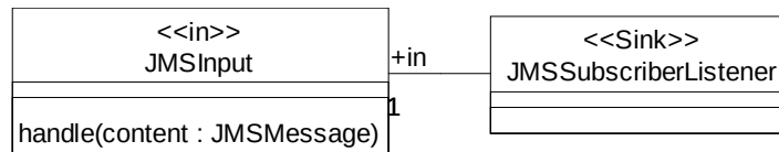
Figure 13-4 A JMSSubscriberListener expects incoming messages
