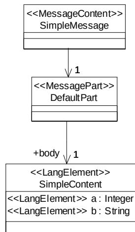
Figure 8-29 A simple message content class
