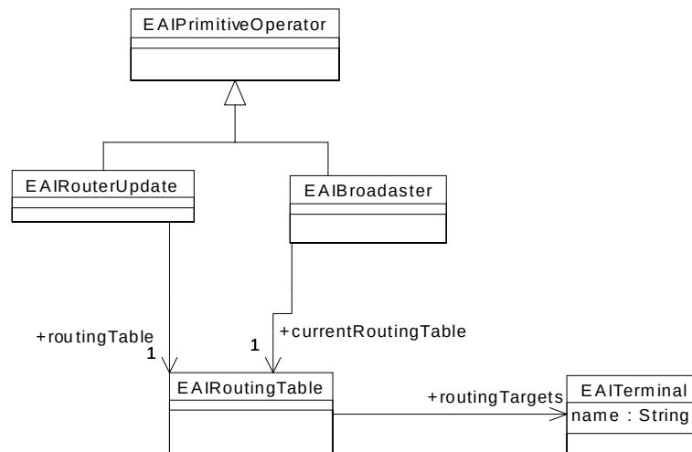
Figure 6-33 EAIRouter and EAIRouterUpdate
