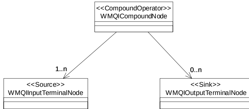
Figure 12-4 Compound and primitive nodes in WMQI
