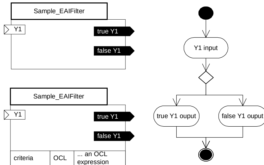
Figure 6-51 CCA notation for a sample EAIFilter
