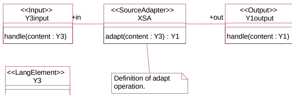
Figure 8-7 Class diagram for prototypical source adapter
