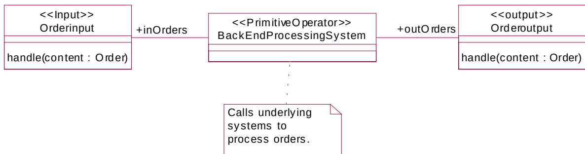
Figure 10-18 Back-end processing system - terminals
