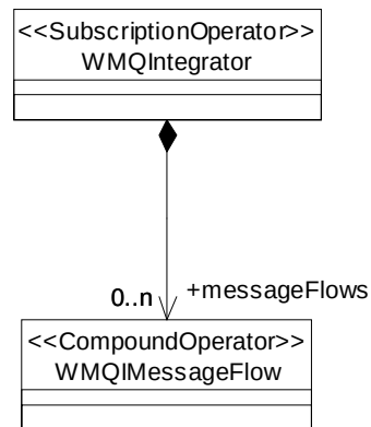
Figure 12-5 WMQIntegrator class diagram
