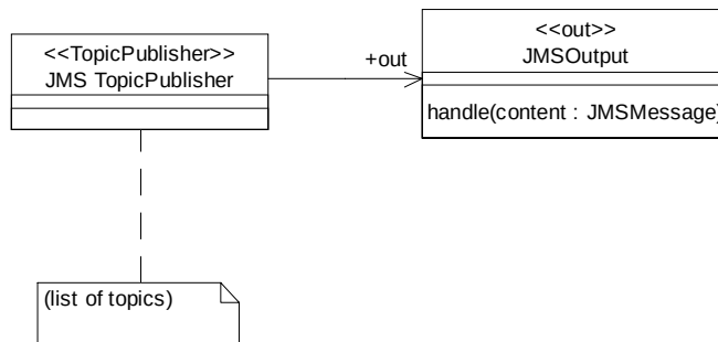
Figure 13-8 A JMS TopicPublisher
