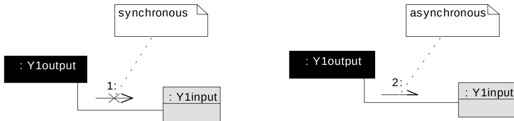
Figure 8-24 Synchronous and asynchronous links
