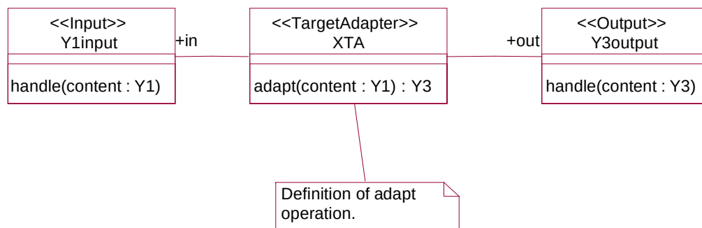
Figure 8-8 Class diagram for prototypical target adapter
