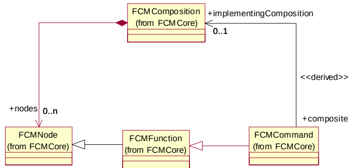
Figure 6-4 Derived association between FCMCommand and FCMComposition
