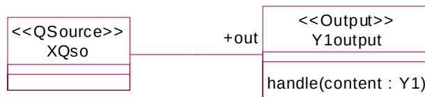
Figure 8-12 Class diagram for prototypical queued source
