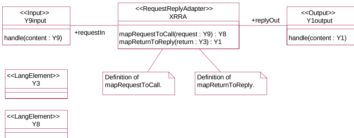
Figure 8-10 Class diagram from prototypical request/reply adapter
