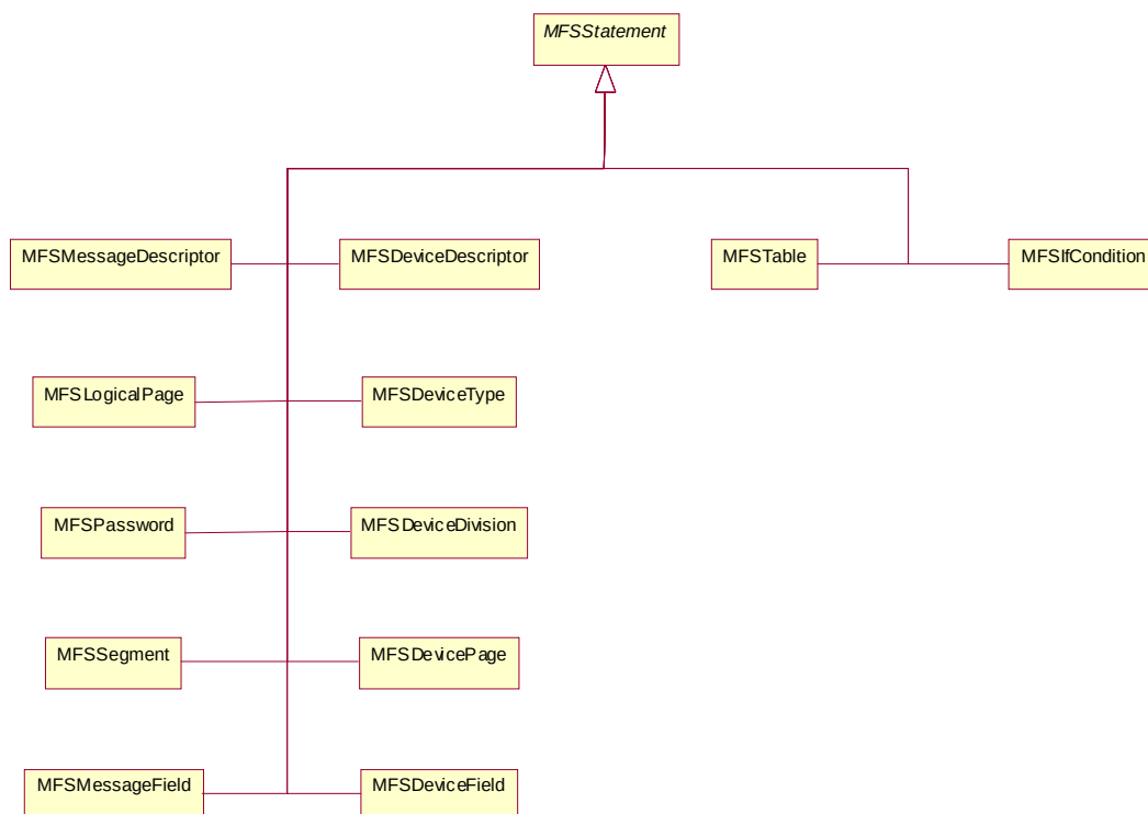
Figure A-7 MFS Inheritance View
