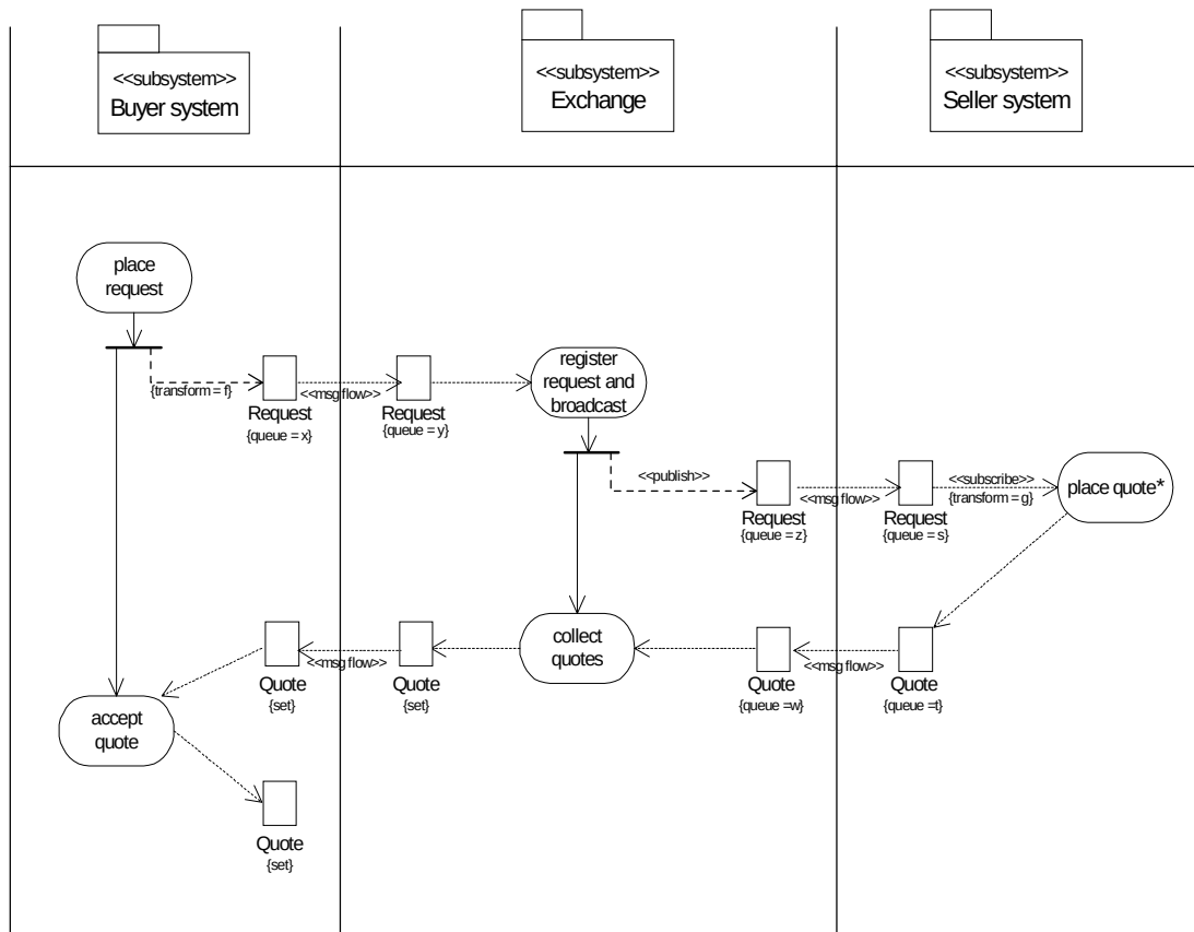
Figure 9-4 Optional control flow transitions between activities within a single system
