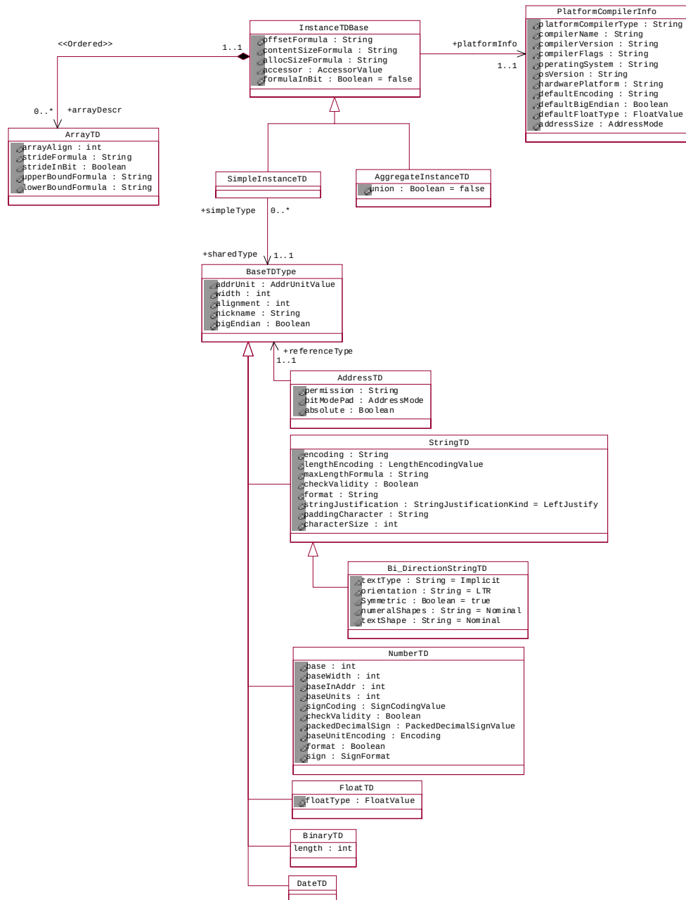
Figure 7-3 Type Descriptor metamodel
