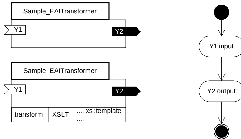
Figure 6-50 CCA notation for sample EAITransformer
