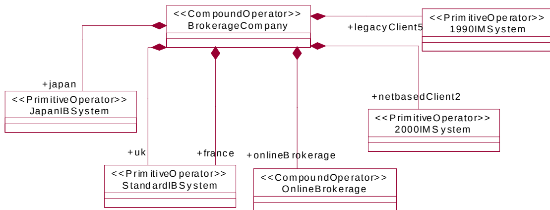
Figure 10-3 Brokerage company - components
