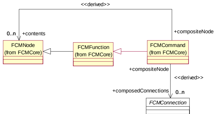
Figure 6-5 Derived association between a composite node, its content nodes and its composed connections
