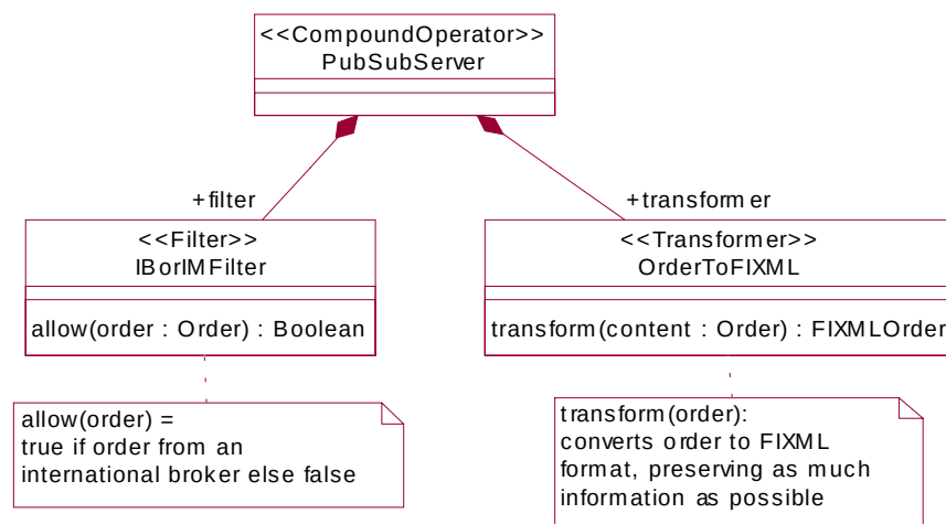
Figure 10-19 Pub/sub server - components
