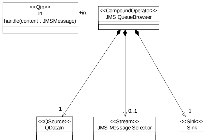
Figure 13-3 JMS QueueBrowser
