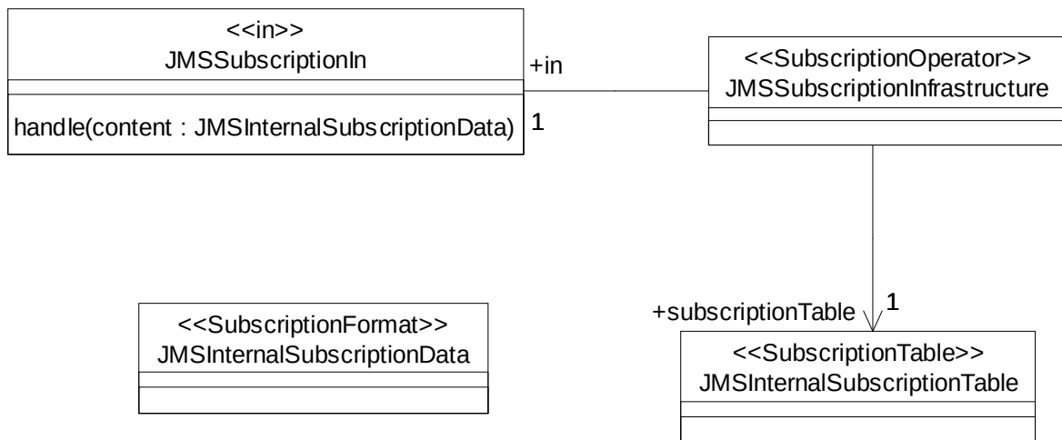
Figure 13-7 JMS SubscriptionInfrastructure
