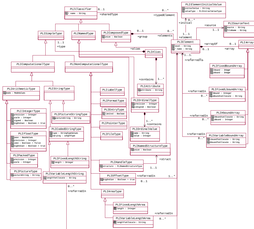
Figure 14-4 PL/I Metamodel
