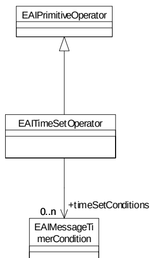
Figure 6-42 TimeSetOperator
