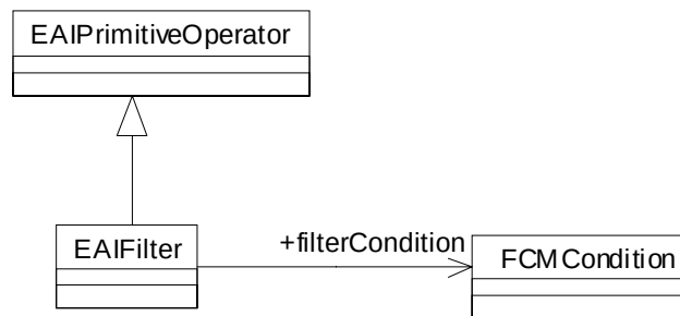
Figure 6-26 Filter
