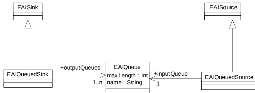
Figure 6-17 QueuedSource and QueuedTarget
