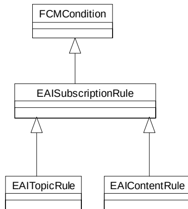
Figure 6-39 EASubscriptionRule, EAITopicRule and EAContentRule
