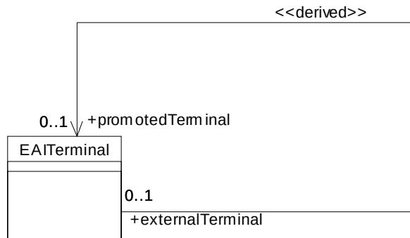
Figure 6-20 Derived association between a terminal inside a composite node and the corresponding terminal outside
