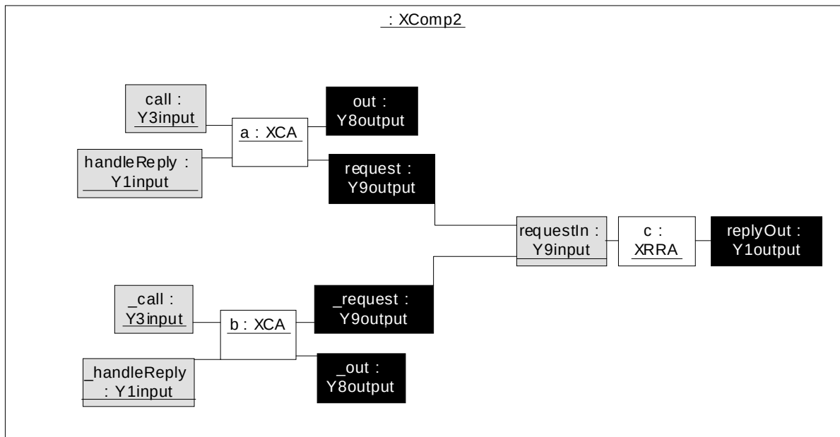
Figure 8-27 Configuration of call and request/reply adapters
