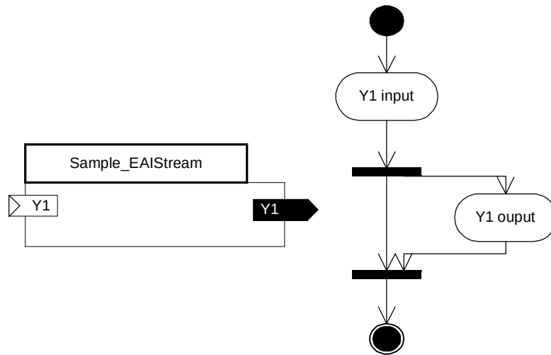
Figure 6-52 CCA notation for a sample EAIStream
