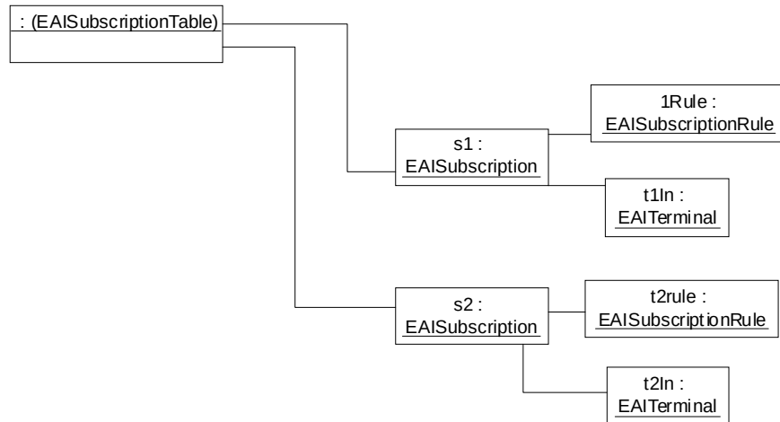
Figure 6-41 Example SubscriptionTable instance diagram
