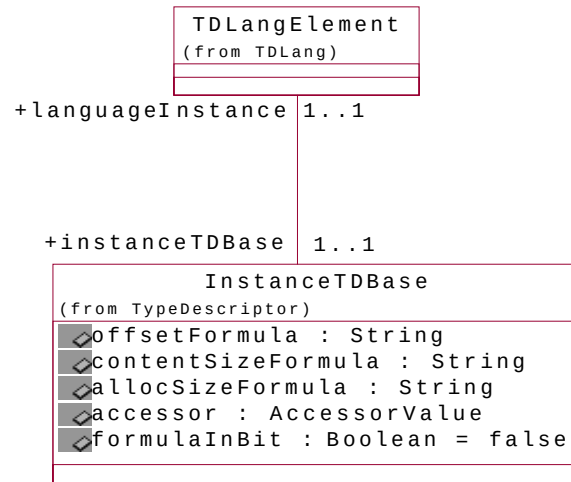
Figure 7-4 TDLang to Type Descriptor
